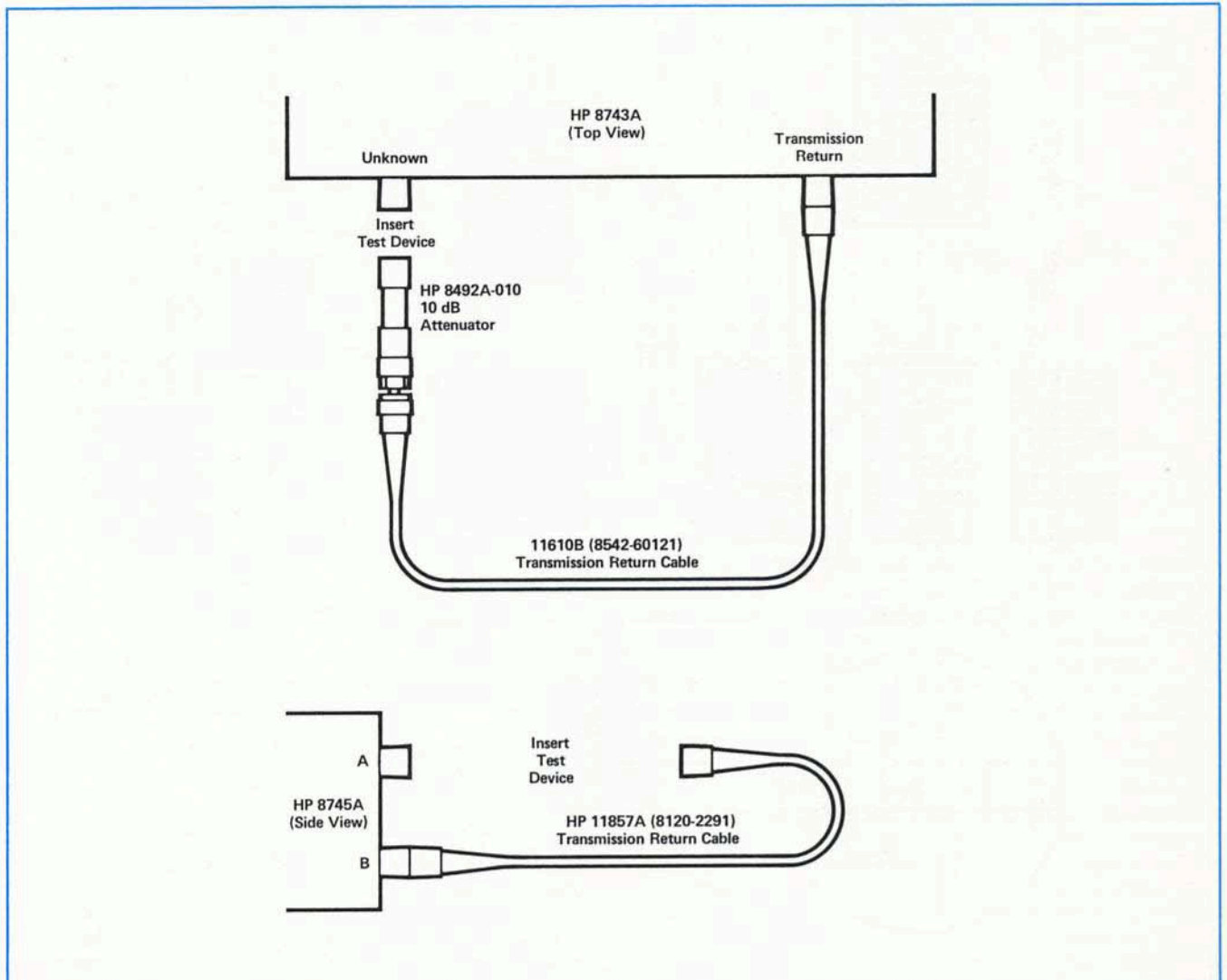
Figure 9. Recommended Transmission Return Cable Configurations for Coaxial Measurements.
