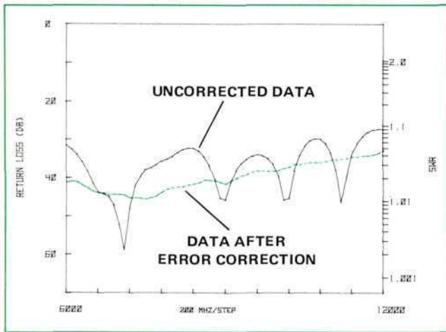
Figure 3. Return Loss Data on a good Termination Before and After Vector Error Correction.
