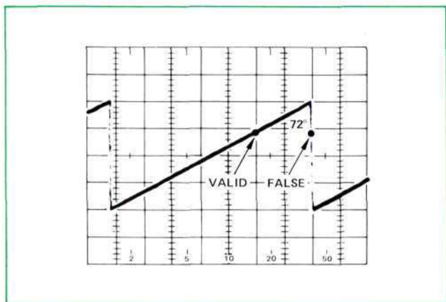
Figure 2. Phase Data is Not Valid if Readings are Taken Within the Transition from +180^\circ to -180^\circ .
