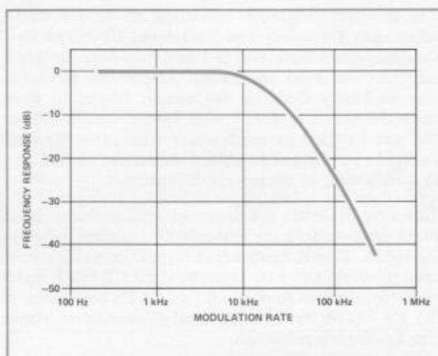
Figure 2. Frequency response resulting from phase modulated 20-30 MHz input signal.
