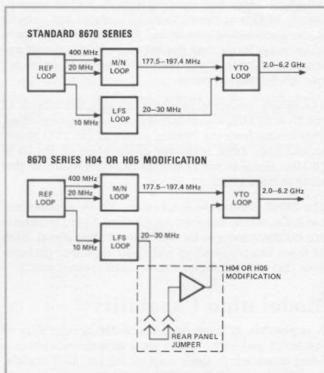
Figure 1. 8670 Series simplified block diagram and block diagram showing H04 or H05 modification.
