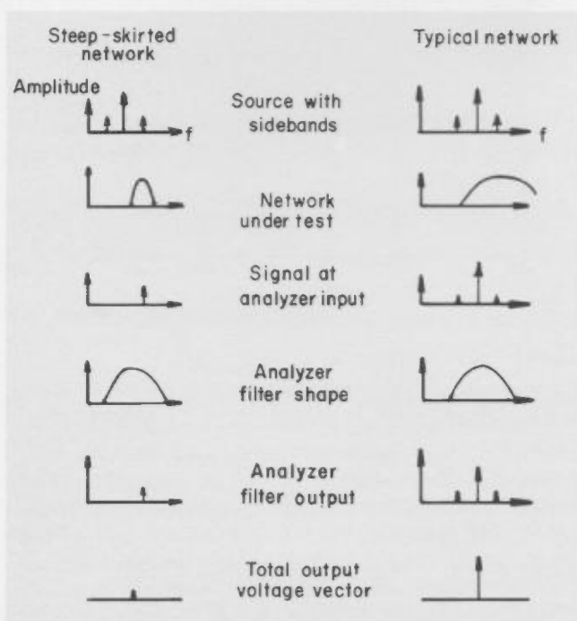
Figure B-2. Effect of oscillator sidebands on network analysis.
