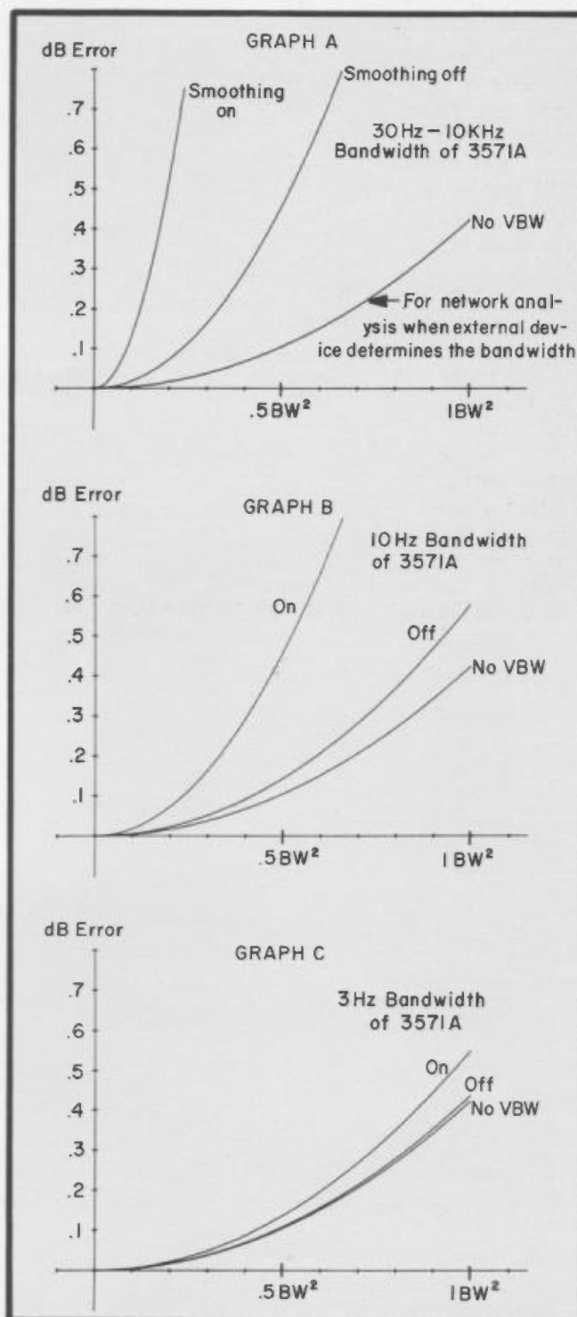
Figure 2.2. Sweep rate versus amplitude compression.
