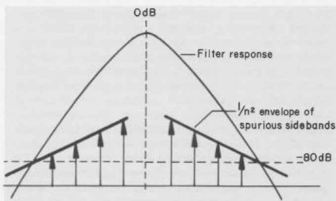
Figure B-4. Case II—first sideband frequency within the 80 dB bandwidth.
