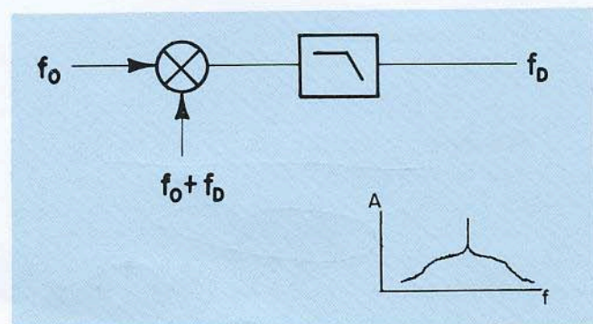
Figure 5. Sideband Translation
