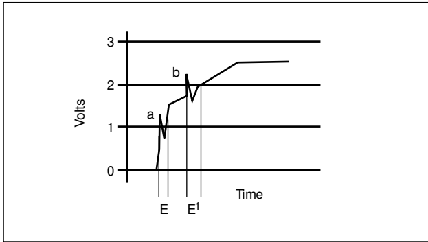
Figure 29. The same amplitude noise pulse gives a smaller error (E) on a fast rise signal (a) than on a slow rise signal (b).
