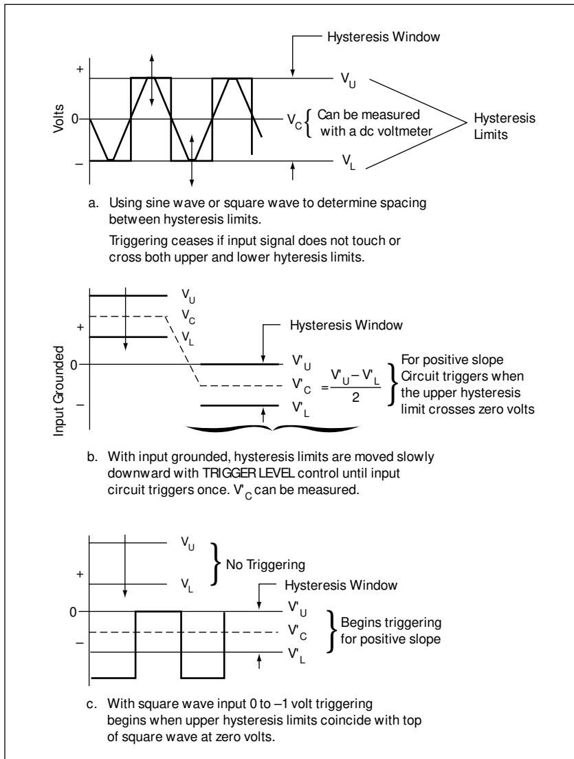
Figure 13. Determining the hysteresis window, i.e., spacing between hysteresis limits, which define the sensitivity of an electronic counter and setting trigger levels at zero volts.
