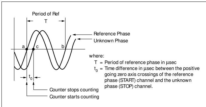
Figure 40. Phase measurement with a time interval counter.
