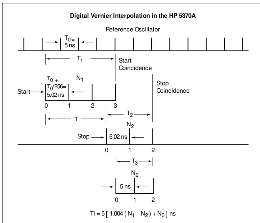
Figure 32. Digital Interpolation Scheme using phase-startable phase-lockable oscillators.
