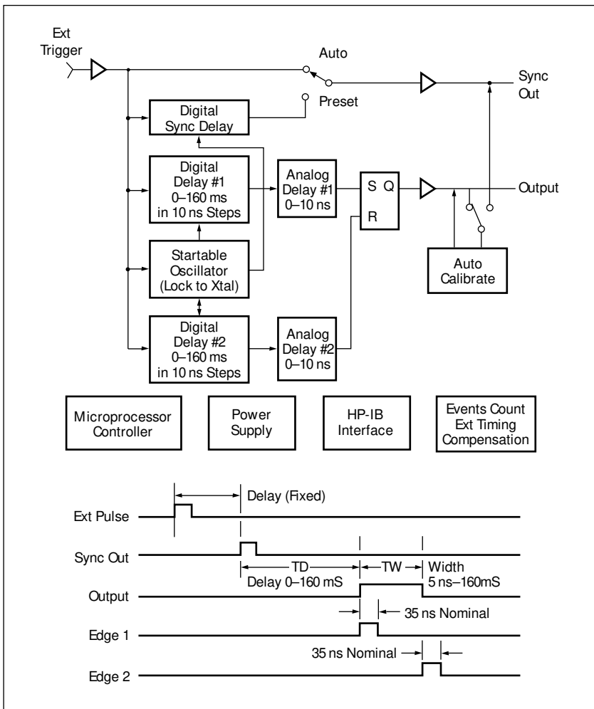
Figure 33. Block Diagram for the HP 5359A Time Synthesizer showing timing relationships between output pulses.
