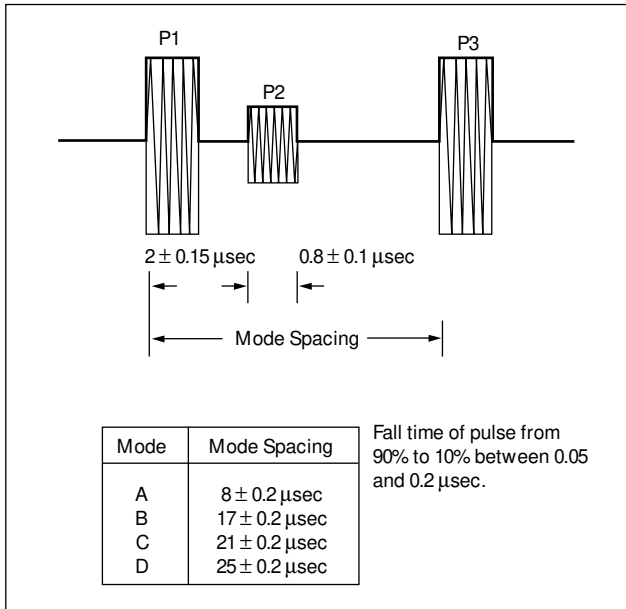
Figure 41. Three-pulse ATC ground station interrogation.
