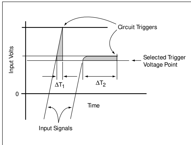
Figure 31. Energy effect introduces time error \Delta T which can be significant on short TI measurement if signal does not extend well beyond the selected trigger point.
