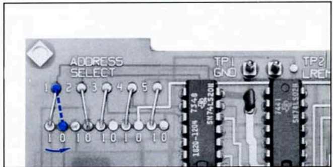
Figure 8. One jumper must be rewired to set the power meter to listen address "L," and talk address "L".
