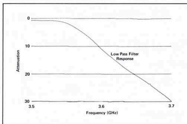
Figure 6. X-Y recorder plot of low-pass filter is made by using the system shown in Figure 5.
