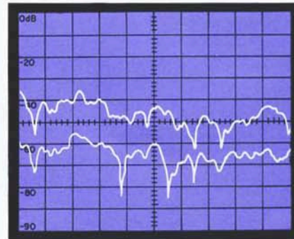
Figure 23. The two response curves (offset by 10dB) show the changes from simply opening a door in the room.
