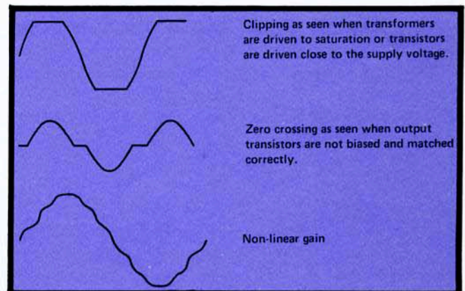
Figure 1. For sine wave inputs, there are three ways that give rise to distortion. The different distortion measurements are designed to expose these effects in different ways.
