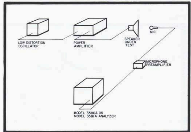
Figure 5. Measuring speaker distortion.
