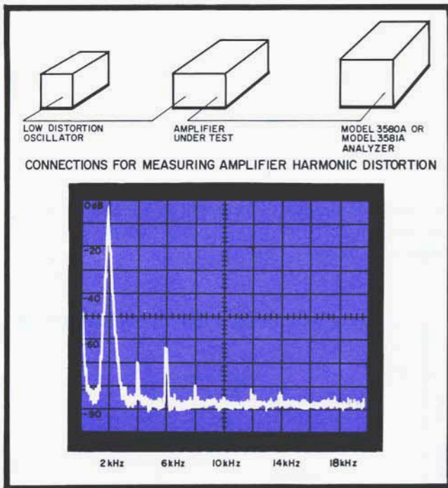
Figure 3. Measurement results show total harmonic distortion to be greater than 63 dB below the fundamental.
