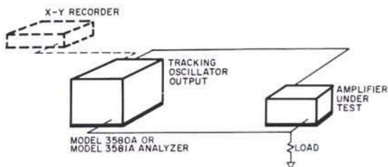
Figure 15. Amplifier frequency response measurement using the Model 3580A or Model 3581A.
