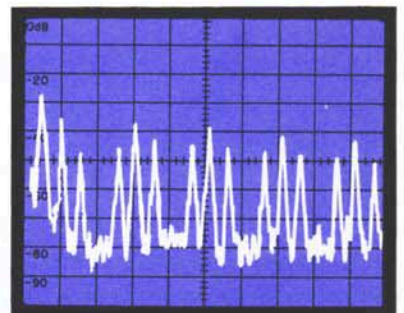
Figure 12. Middle C with a violin voice.
