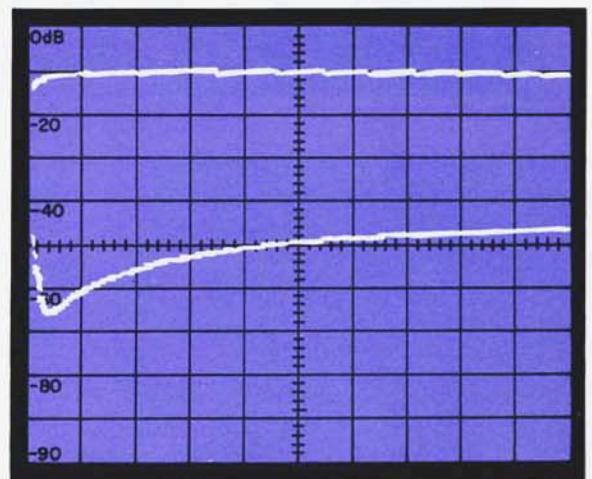
Figure 26. Cross-talk over entire frequency.
