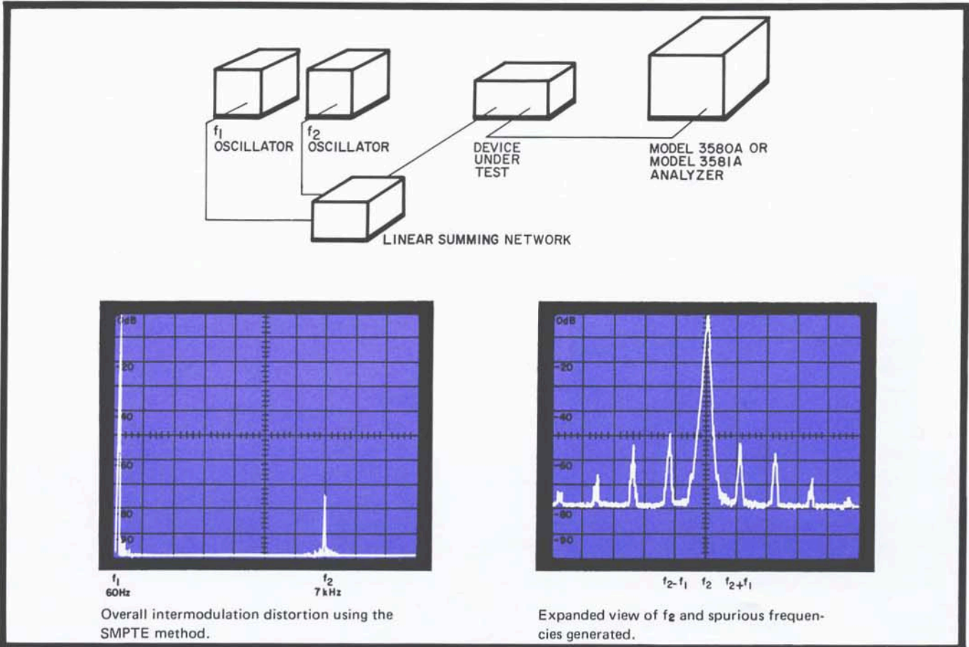
Figure 6. Test connections and measurement results for SMPTE intermodulation distortion.
