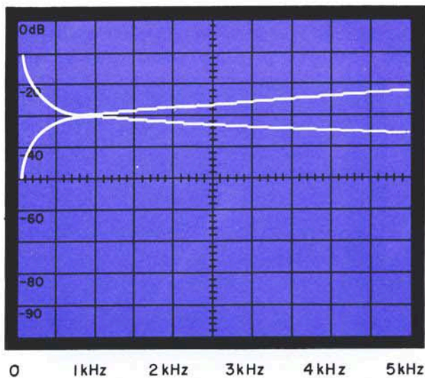
Figure 16. Bass and treble controls effect on the frequency response of an amplifier.
