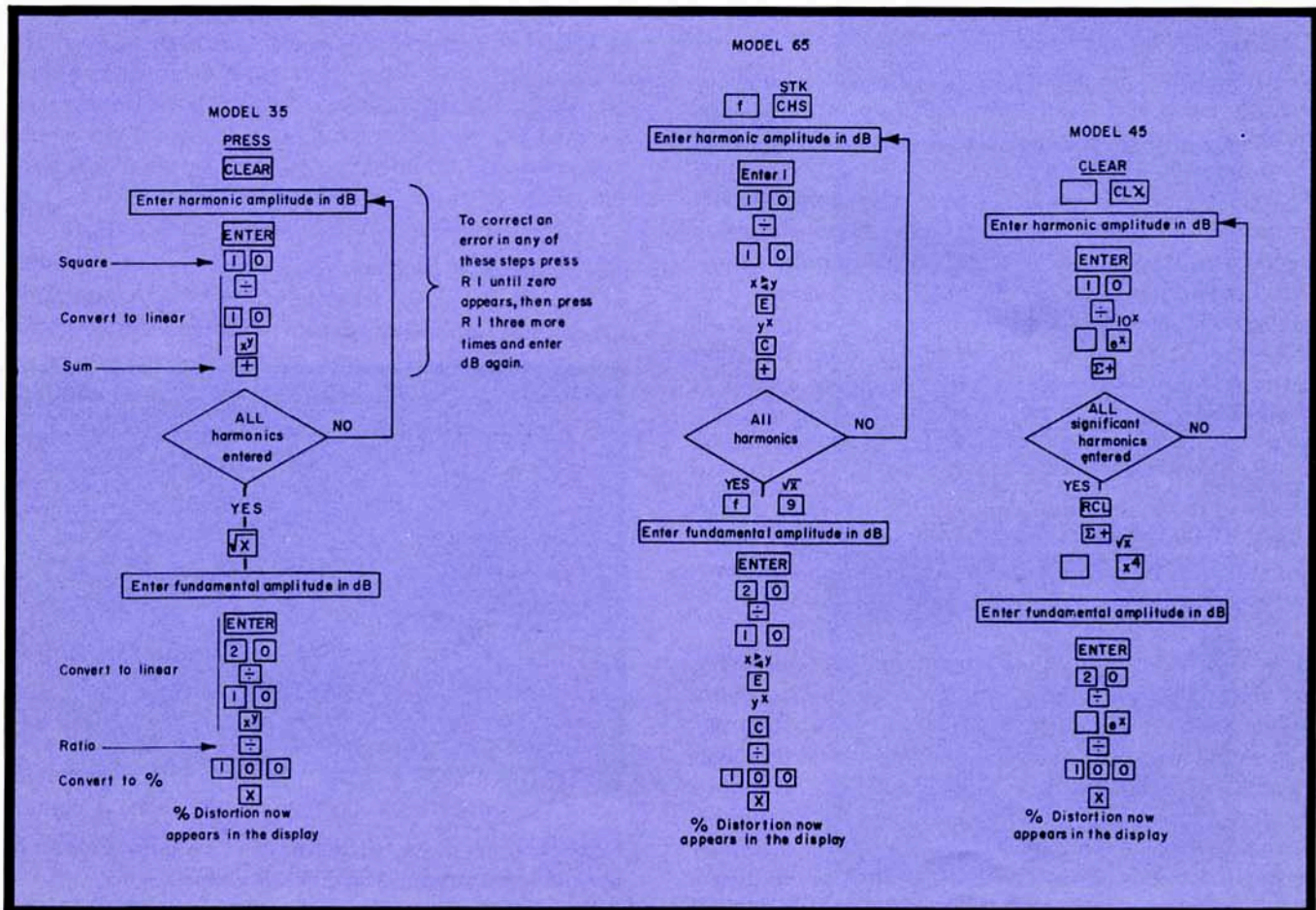
Figure 2. Three harmonic distortion algorithms using HP calculators.
