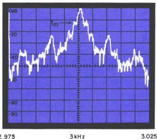
Figure 8. Flutter and wow measurement with the Model 3580A.
