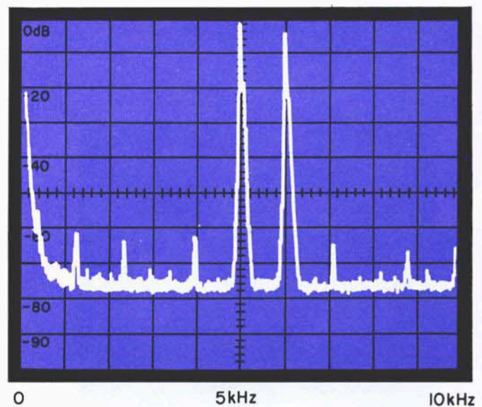
Figure 7. Distortion measurement using the CCIF method.
