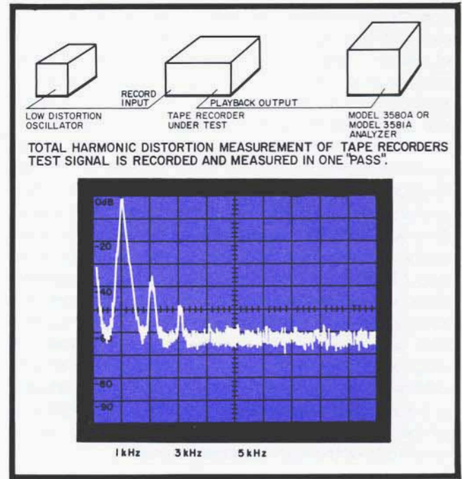
Figure 4. Total harmonic distortion of tape recorder shows THD to be approximately 2%.
