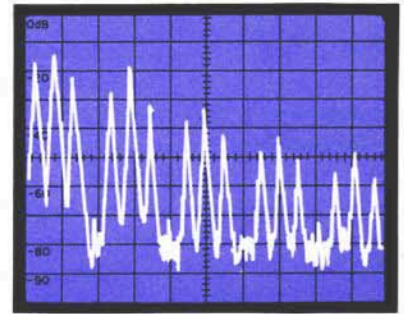
Figure 10. The harmonics of Middle C.
