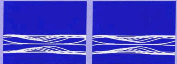
Figure 19. Shelving equalizer family of curves for two separate equalizers. 10 dB/vertical cm with horizontal reference times at \pm 10 dB and \pm 12 dB, log frequency sweep, 20 Hz to 43 kHz.
