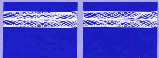
Figure 20. Peaking and notching curves for two separate equalizers. 10 dB/vertical cm with horizontal reference lines at \pm 10 and \pm 12 dB, log sweep, 20 Hz to 43 kHz.
