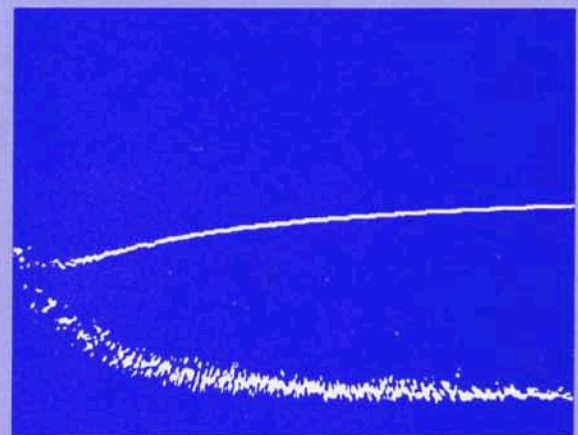
Figure 27. Adjacent channel cross talk (upper trace), and channel residual noise (lower trace). 10 dB/vertical cm. 5 kHz/horizontal cm (linear sweep).
