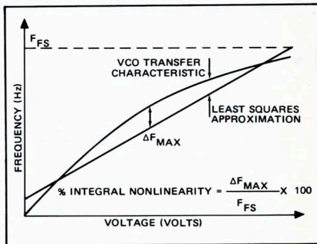
Figure 2. Definition of Integral Nonlinearity for VCO
