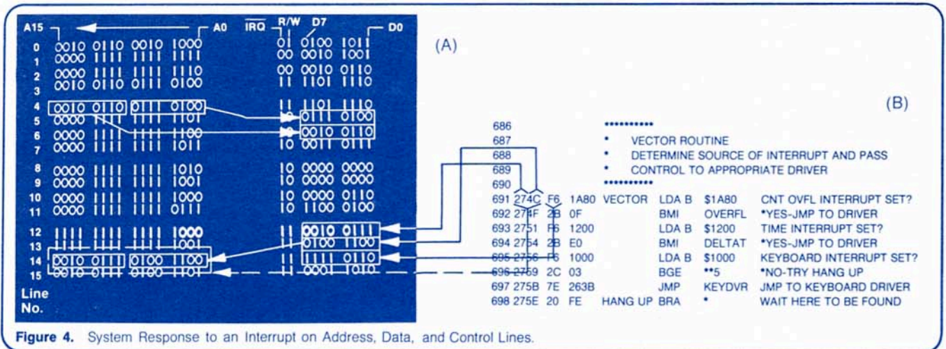
Figure 4. System Response to an Interrupt on Address, Data, and Control Lines.
