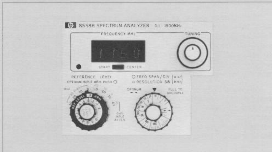
Figure 4-1. Three knob settings for simple operation.
