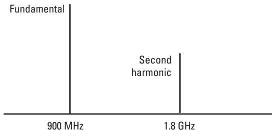
Figure 5. Fundamental and second harmonic in the same frequency band
