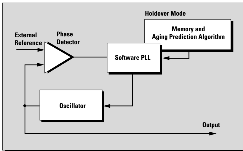
Figure 1. HP SmartClock Technology includes algorithms for steering the oscillator. The frequency is corrected to compensate for the effects of aging and temperature.
