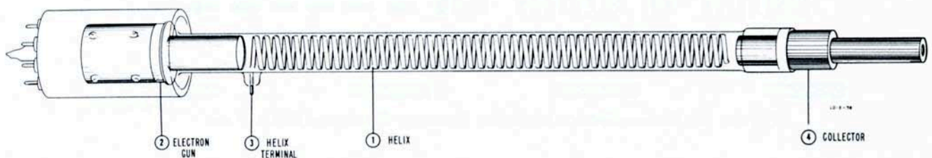
Figure 1. Backward Wave Oscillator Tube
