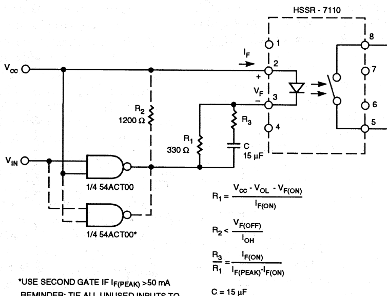
Figure 8. Peaking to Shorten Turn-on Time.
