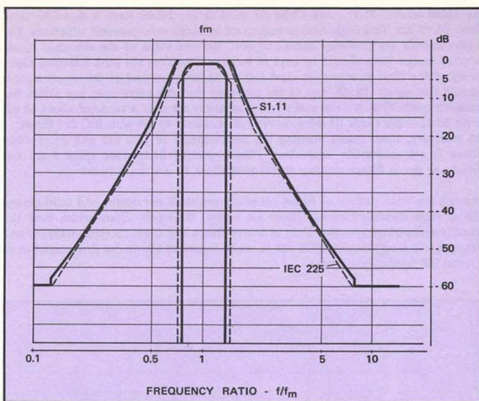
Figure 40. Class II octave filter transmission characteristics
