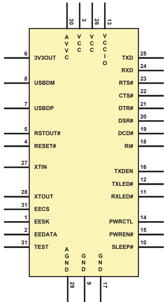
Figure 2 Pin-Out (Schematic Symbol)
