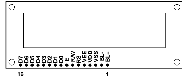
LCD 1602D
