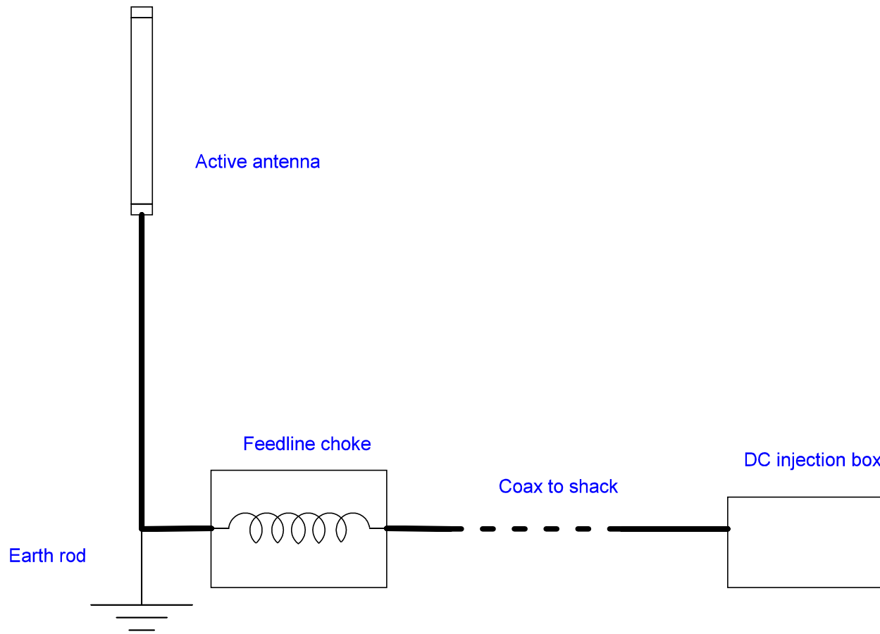
General installation of a PA0RDT antenna
