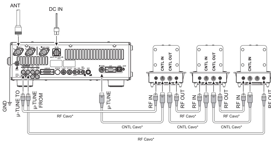
RF Cavo*
