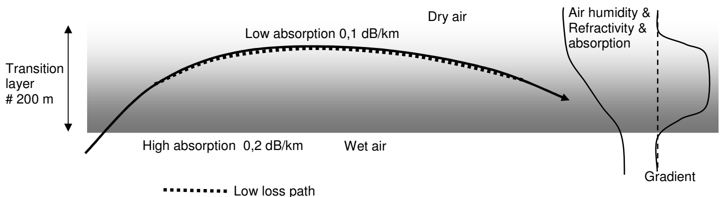
Figure 17 : Propagation across a transition layer
