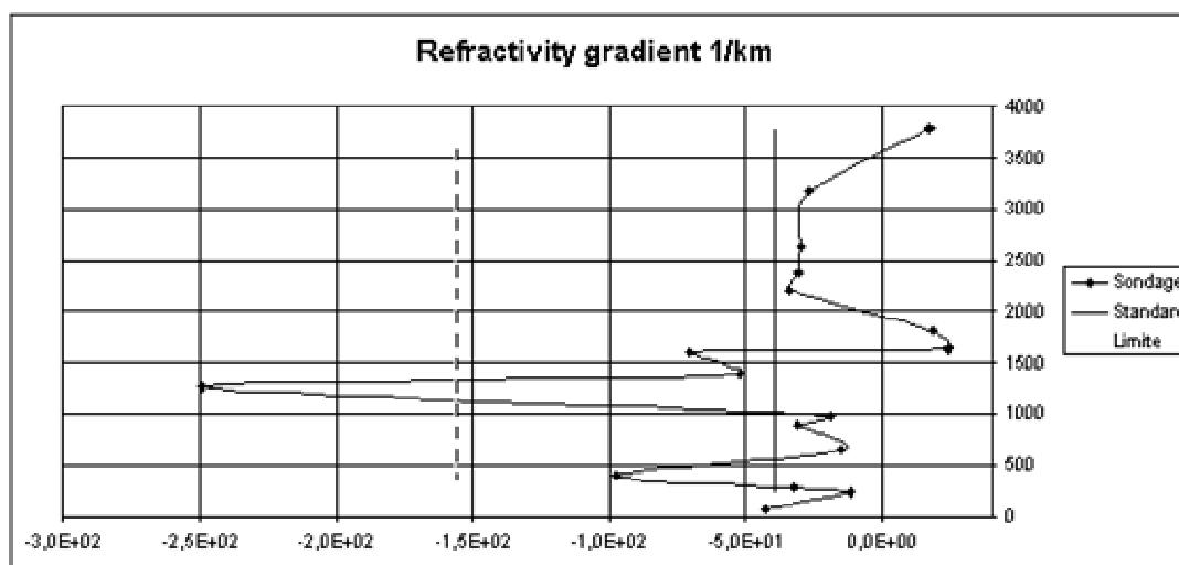
Figure 9 : Air refractivity gradient profile (12H00 TU)
