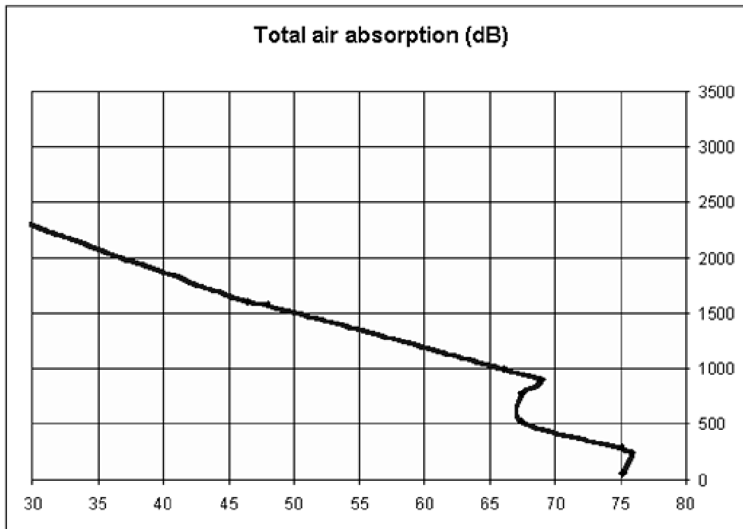
Figure 6 : Air absorption profile at 47 GHz (00H00 TU)
