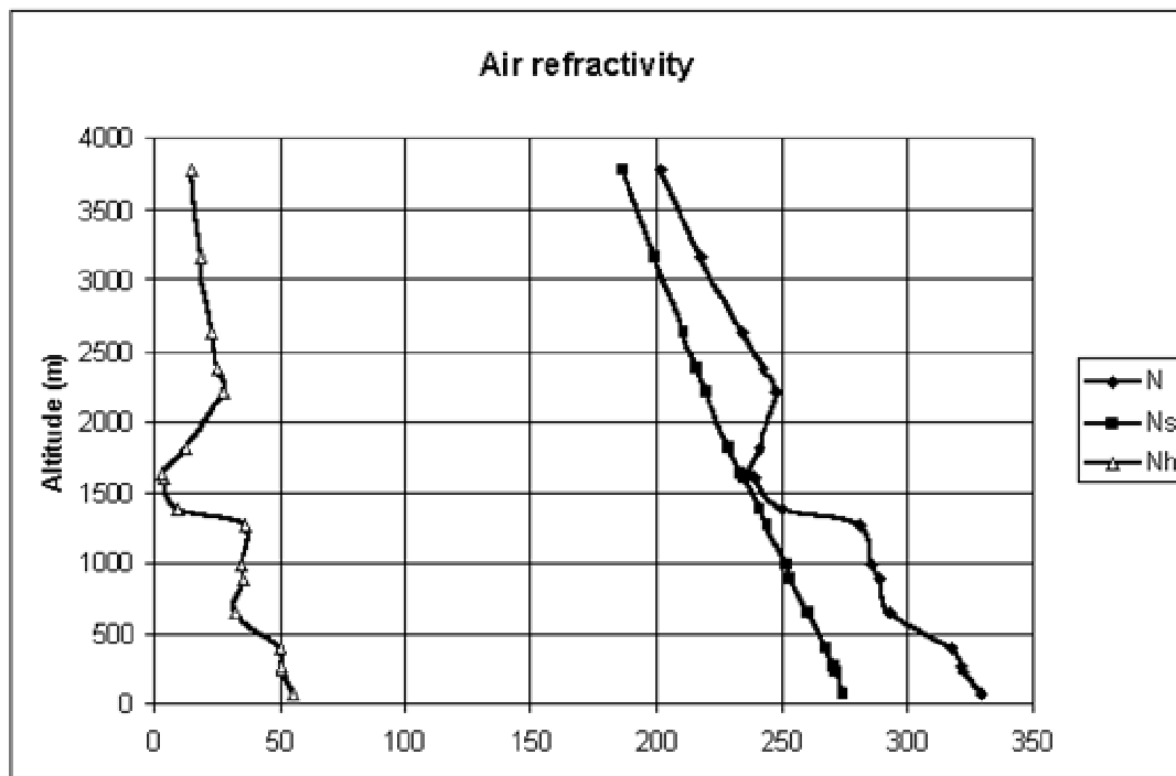
Figure 8 : Air refractivity profile ( N_s = N_{\text{dry}} N_h = N_{\text{wet}} ) (12H00 TU)
