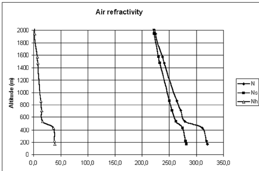
Figure 13 : Air refractivity profile ( N_s = N_{\text{dry}} N_h = N_{\text{wet}} ), Trappes (00H00 TU)
