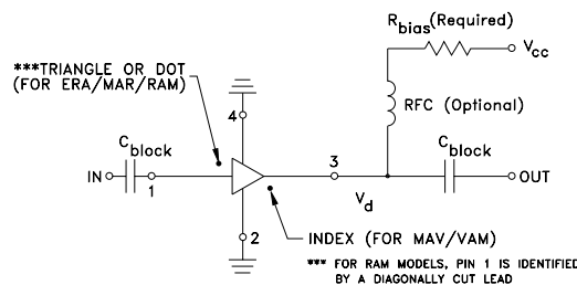
typical biasing configuration ERA/MAR/MAV/RAM/VAM
