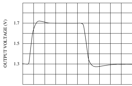
Small Signal Pulse Response (Single Supply)
