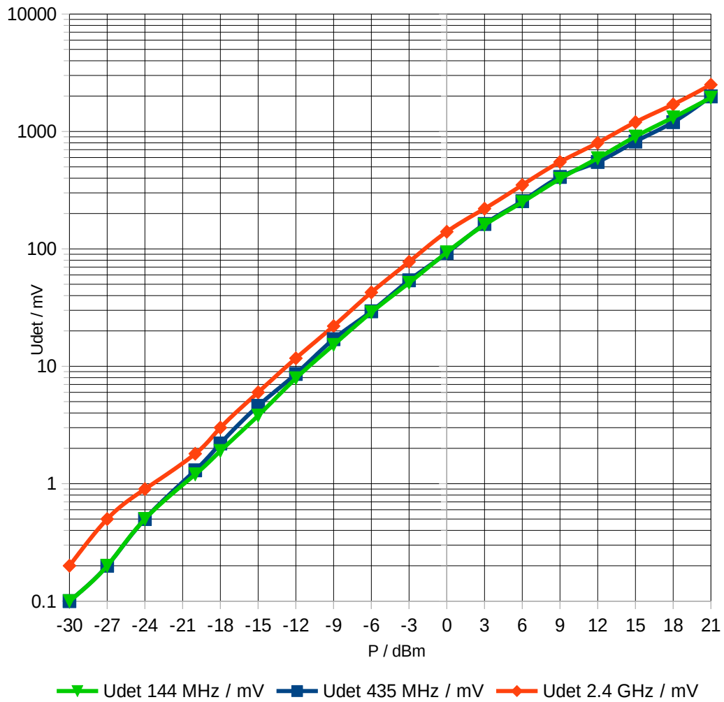
Diode Probe Calibration
