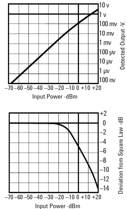
Figure 1. The diode detection characteristic ranges from the square-law region through a transition region to linear detection.
