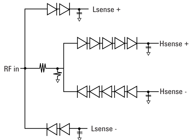
Figure 2. Schematic of the diode-attenuator-diode sensing element
