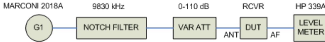
BLOCK DIAGRAM OF RECIPROCAL MIXING TEST SETUP
