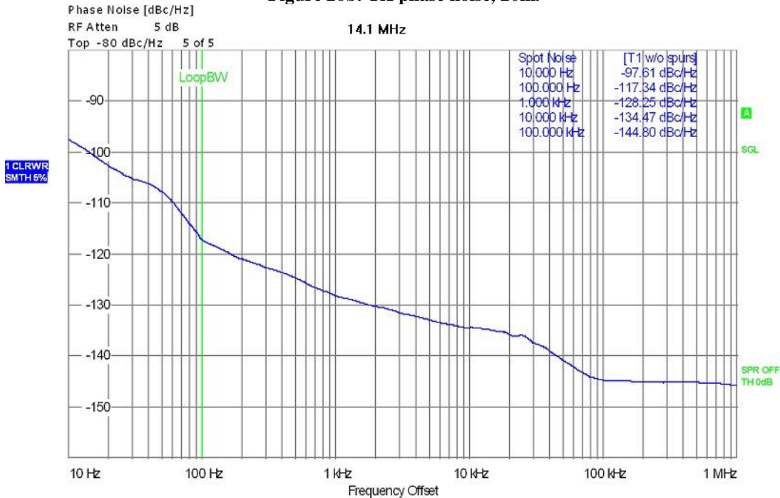
Figure 26b: TX phase noise, 20m.
