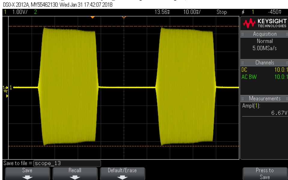
Figure 29: Keying envelope at 48 wpm, 2 ms rise time.
