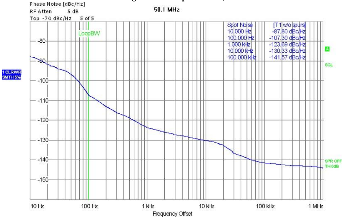
Figure 26d: TX phase noise, 6m.
