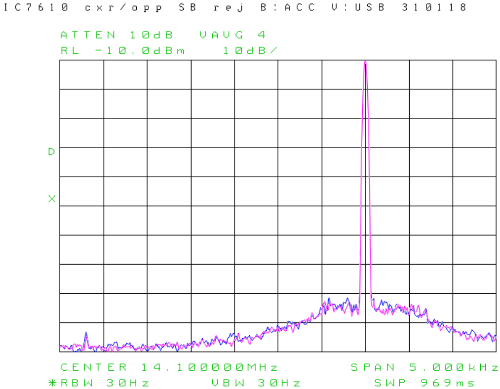
Figure 34: Carrier & opposite-sideband suppression at 14.1 MHz.
