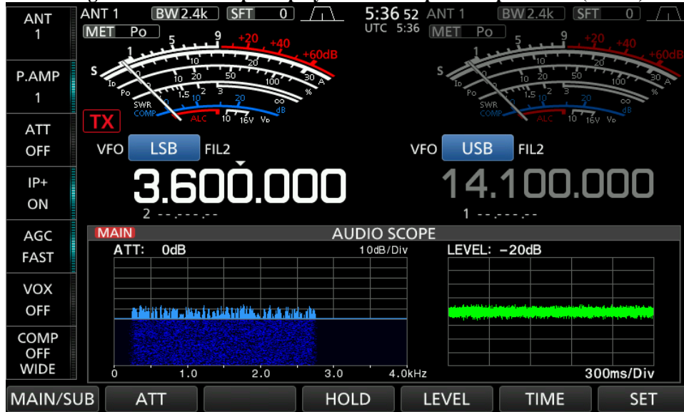
Figure 4b: Audio scope display for AGC impulse response test (NB on).
