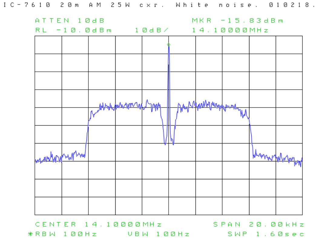
Figure 35: AM with white noise modulation.
