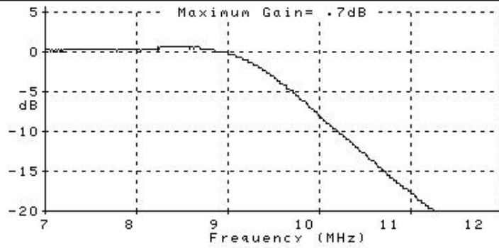
Fig. 4: Swept Gain, 40m.
