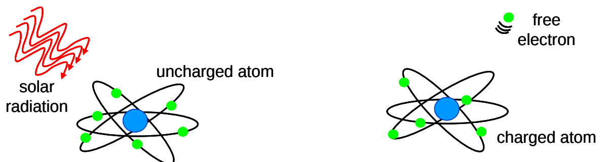
Figure 1.2 Free electron production in the ionosphere
