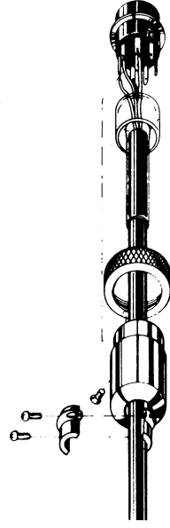
Microphone plug exploded view
