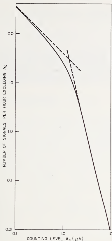
FIGURE 8.9. Theoretical rate-amplitude relation computed for the following parameters: P_t = 100 W , \lambda = 7.5 m , g_i = g_r = 40 .
