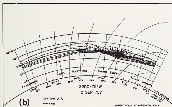
FIGURE 3.18—Continued. Ionospheric sections along the 75th geographic meridian.
