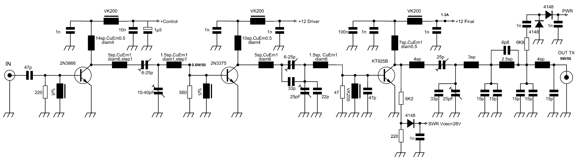
FRONT END MOSFET 144-146MHZ POWER AMPLIFIER FM 9W YO4HFU
