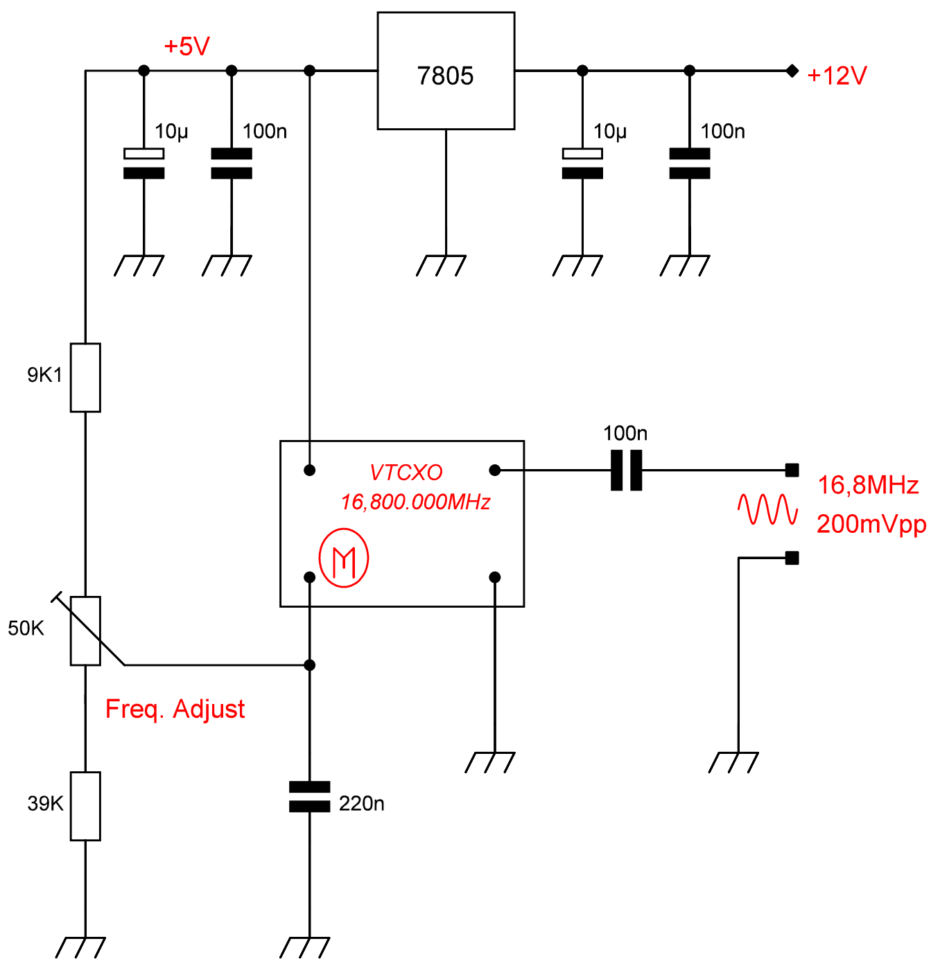
REFERENCE OSCILLATOR FOR RDDS YO4HFU (2012)
