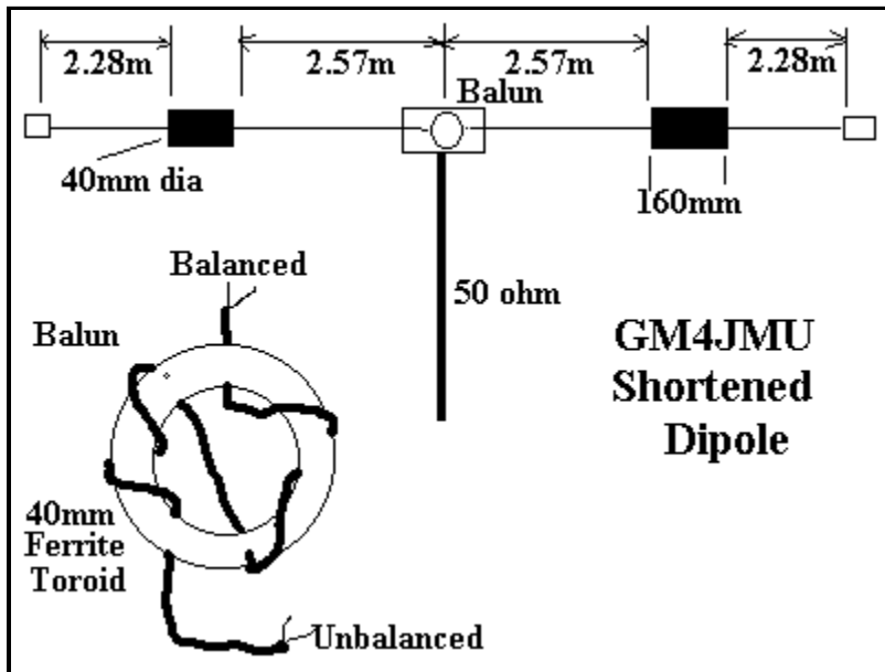
The GM4JMU Shortened 7Mhz
