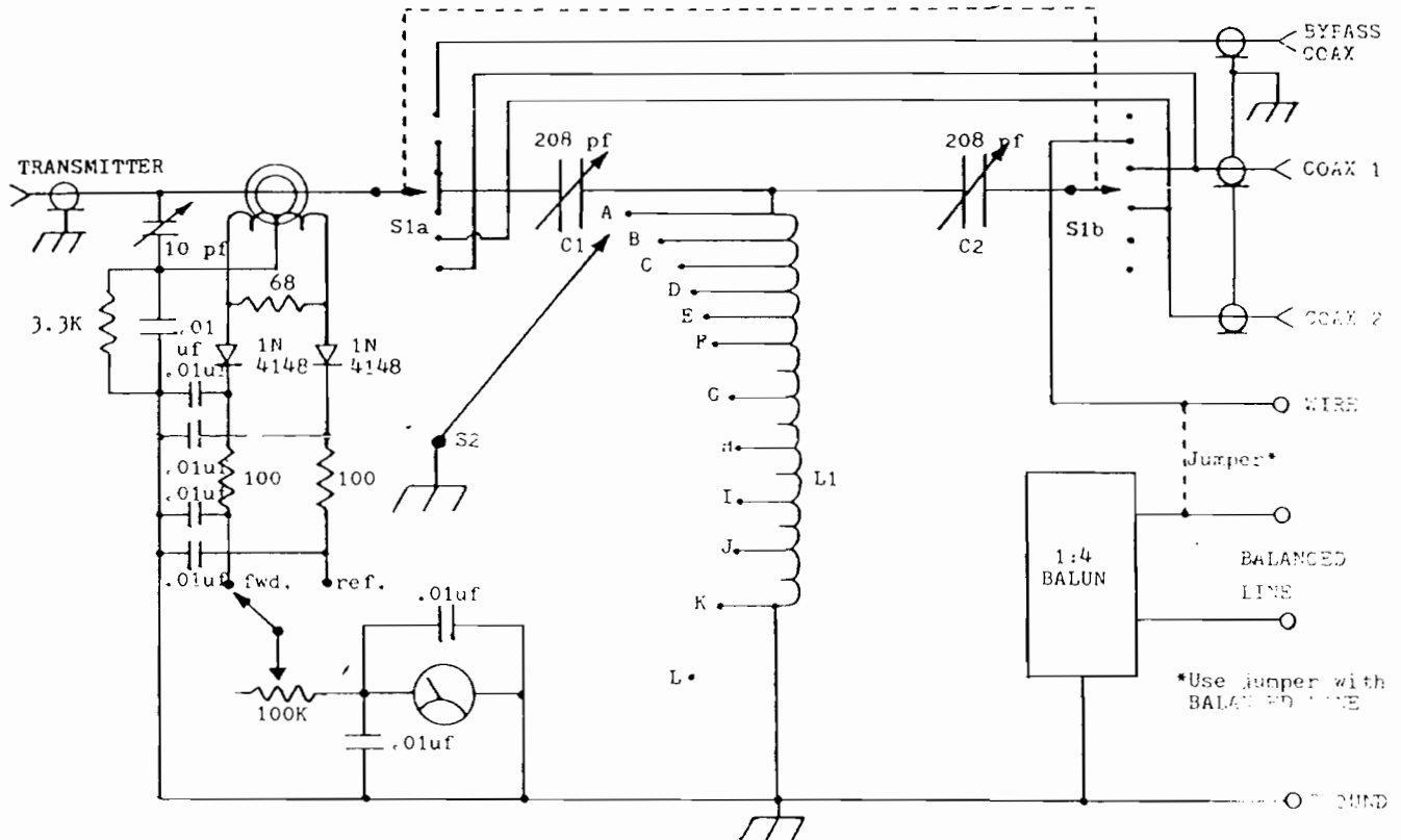
MFJ-941C SCHEMATIC DIAGRAM
