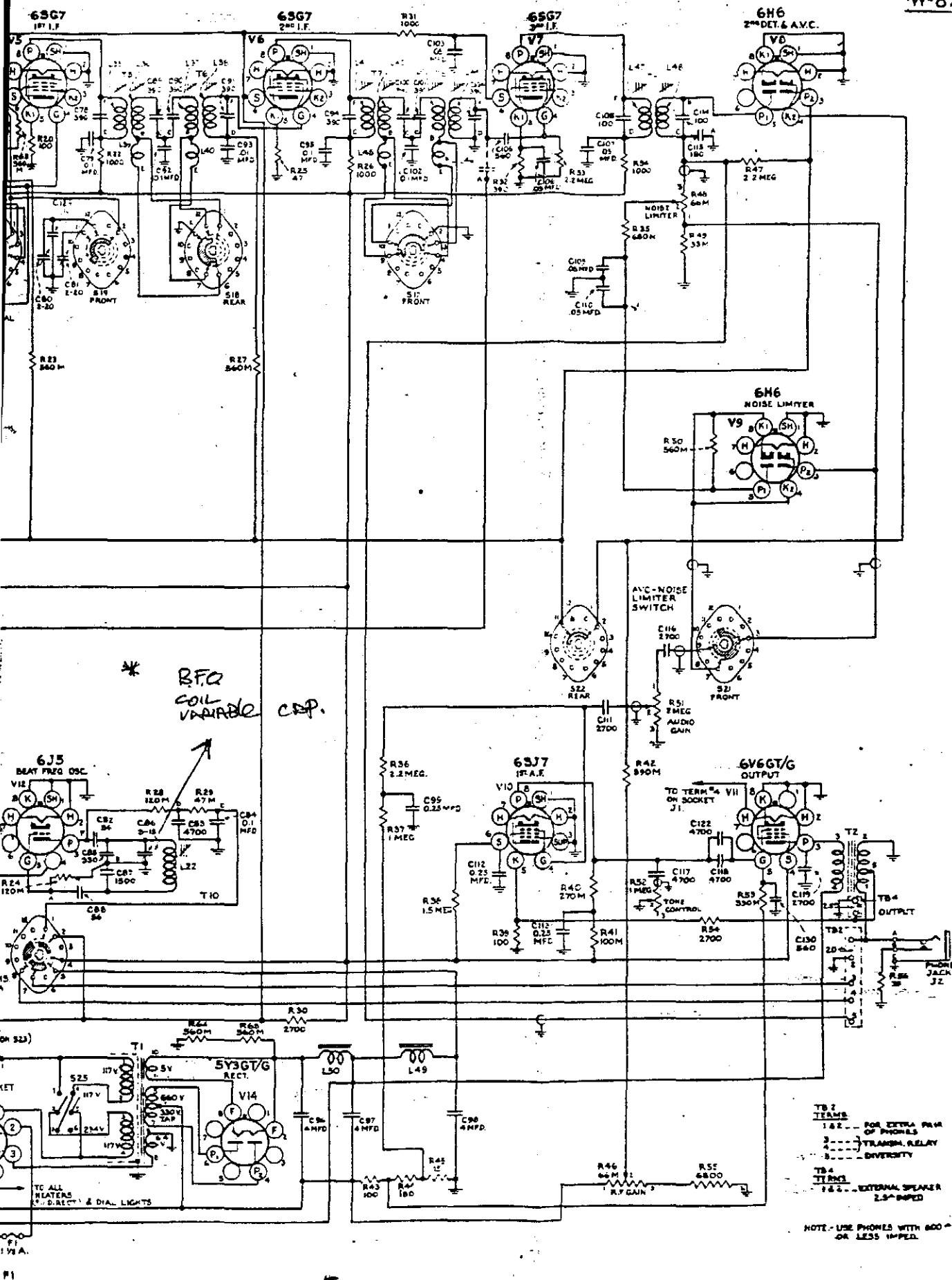
Figure 11.—General Purpose Communications Receiver — Schematic Diagram.
