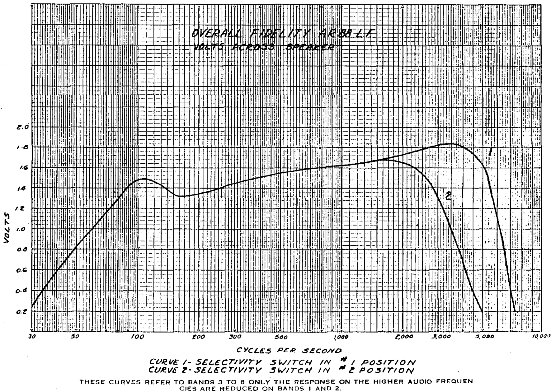
Figure 13.—General Purpose Communications Receiver—Fidelity Characteristics. [34]
