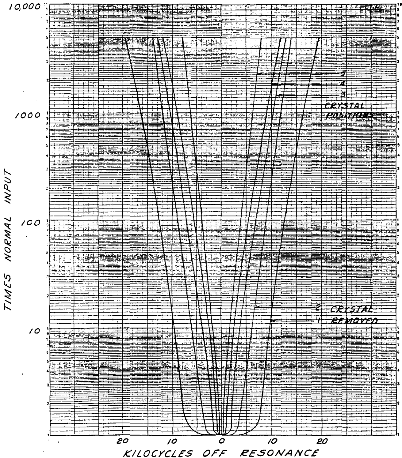
Figure 12.—General Purpose Communications Receiver—Selectivity Characteristics.
