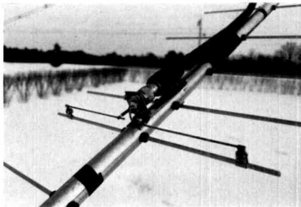
Photo A. Thirty-two element Yagi driven element.
