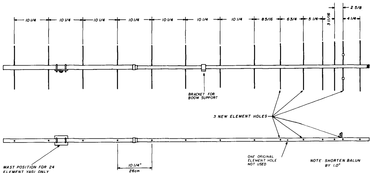
fig. 10. New spacing pattern for 24, 32, and 38-element Yagi.
