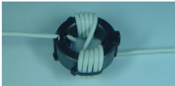
400 Watt Balun
