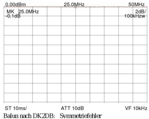
1 KW Balun
