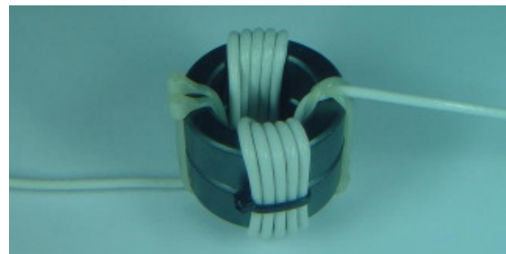
1 KW Balun
