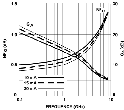
Figure 1. ATF-21186 Optimum Noise Figure and Associated Gain vs. Frequency and I_{DS} , V_{DS} = 2 V.
