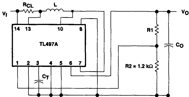
BASIC CONFIGURATION (Peak Switching Current = I_{(PK)} < 500 mA)
