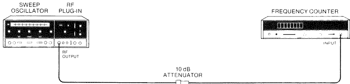
Figure 2-3. Frequency Range and Accuracy Test Setup
