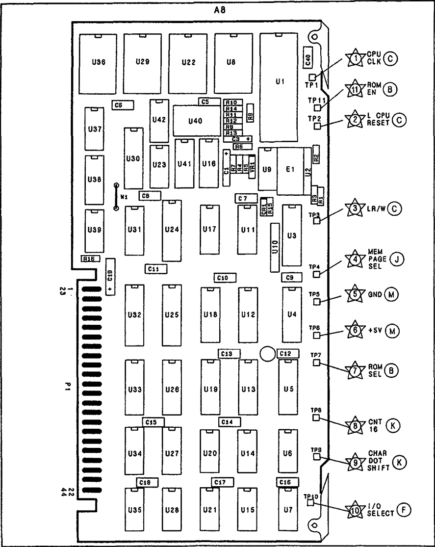
Figure 8-28. A8 Microprocessor Assembly, Component Locations
