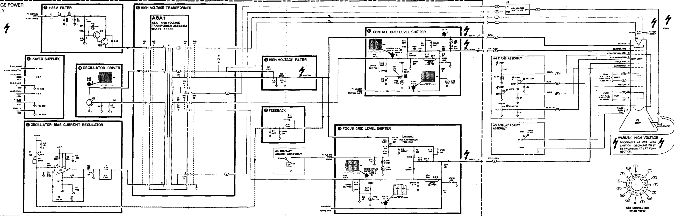
Figure 8-20. A6 High Voltage Power Supply Assembly, Schematic Diagram
