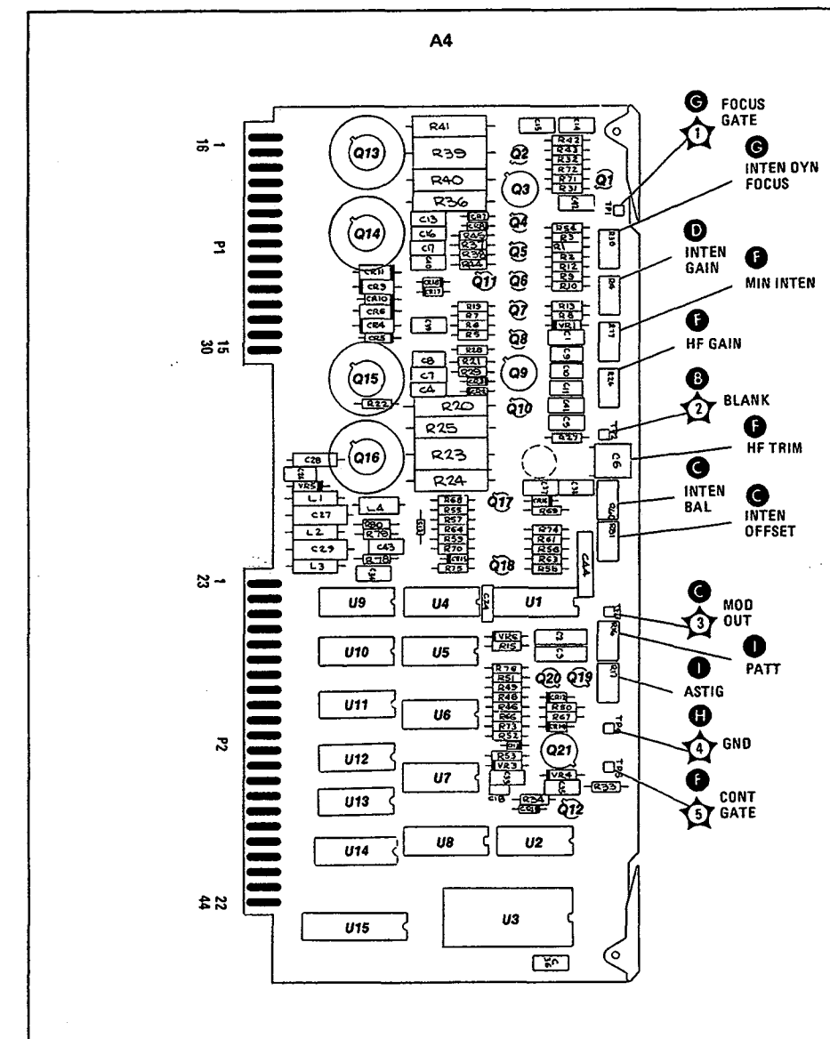
Figure 8-15. A4 Z Axis Assembly, Component Locations
