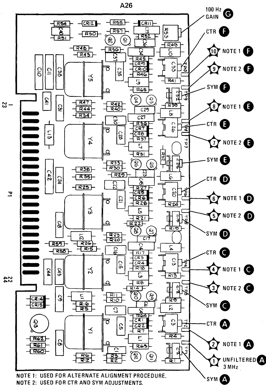
Figure 8-85. A26 3 MHz Filter Assembly, Component Locations
