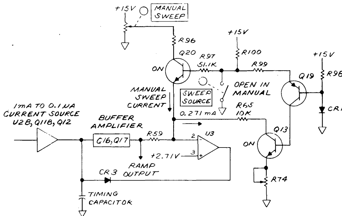
Figure 8-52. Manual Sweep, Simplified Schematic Diagram
