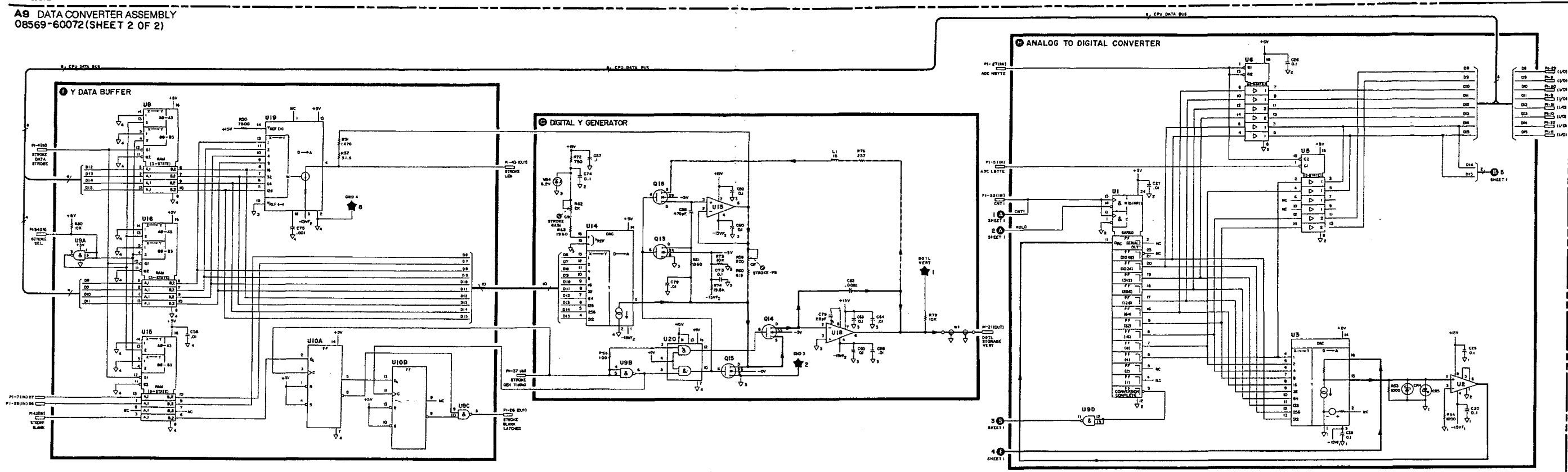
Figure 8-32. A9 Data Converter Assembly, Schematic Diagram (2 of 2)
