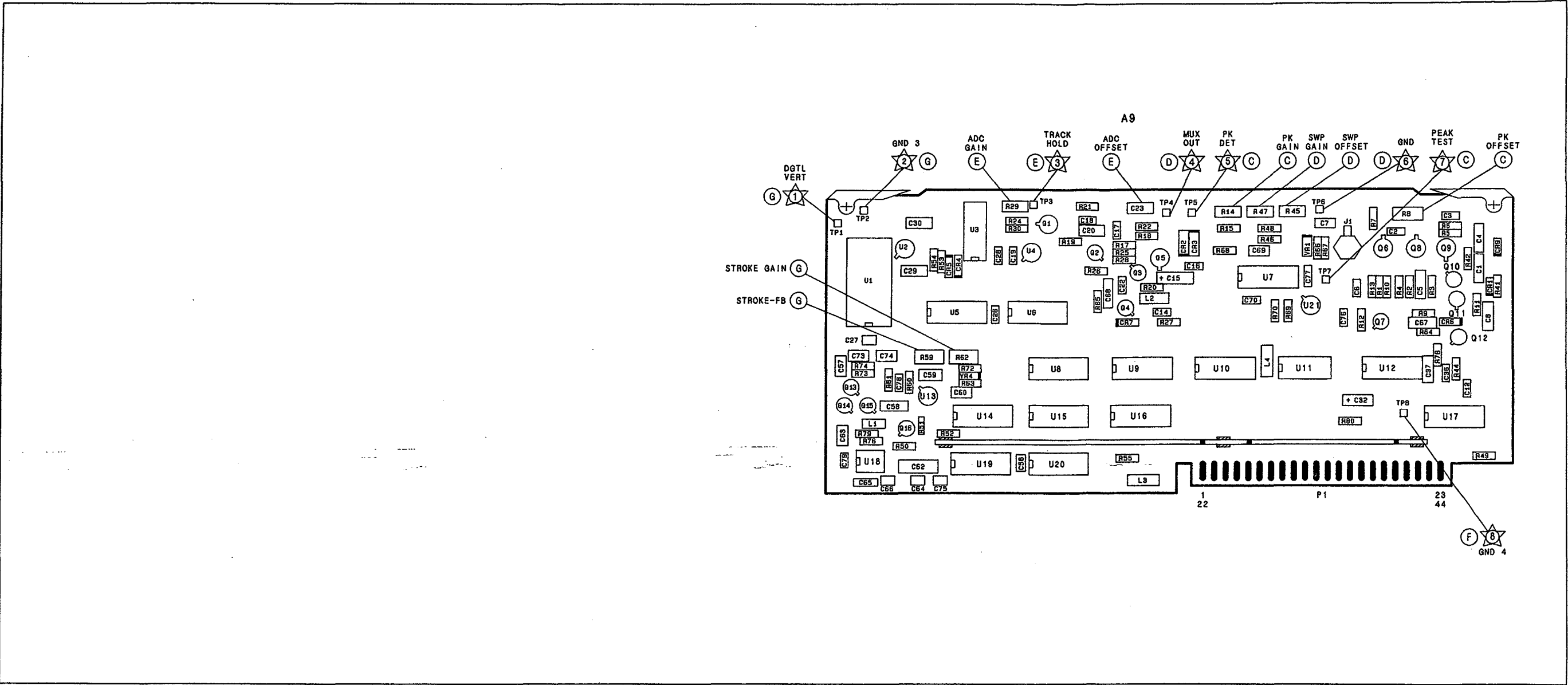
Figure 8-31. A9 Data Converter Assembly, Component Locations
