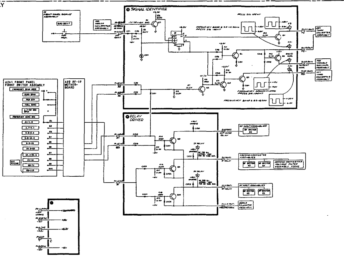
Figure 8-43. A13 Relay Driver Assembly, Schematic Diagram
