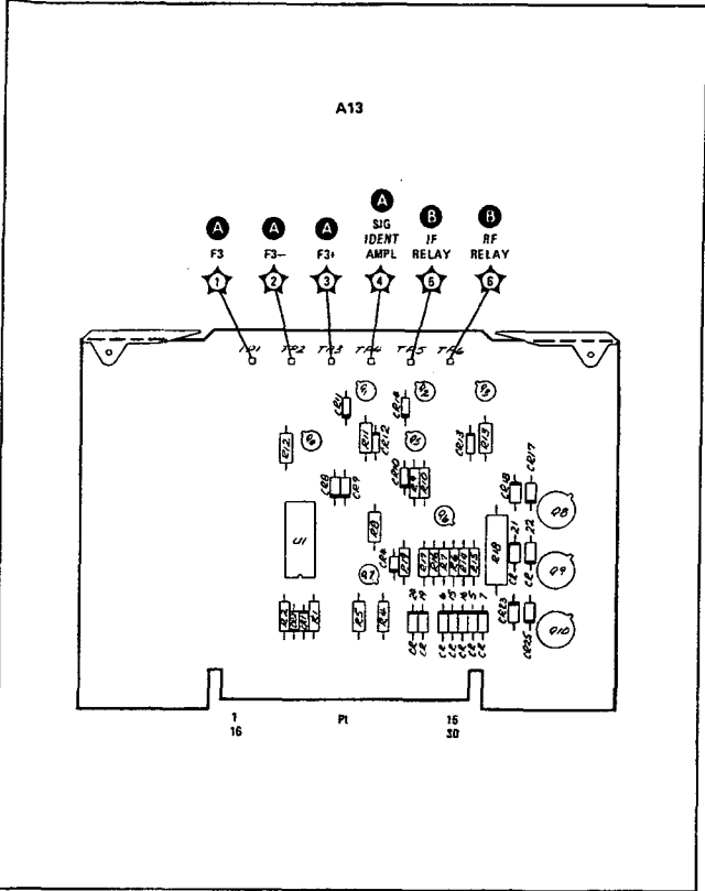
Figure 8-42. A13 Relay Driver Assembly, Component Locations
