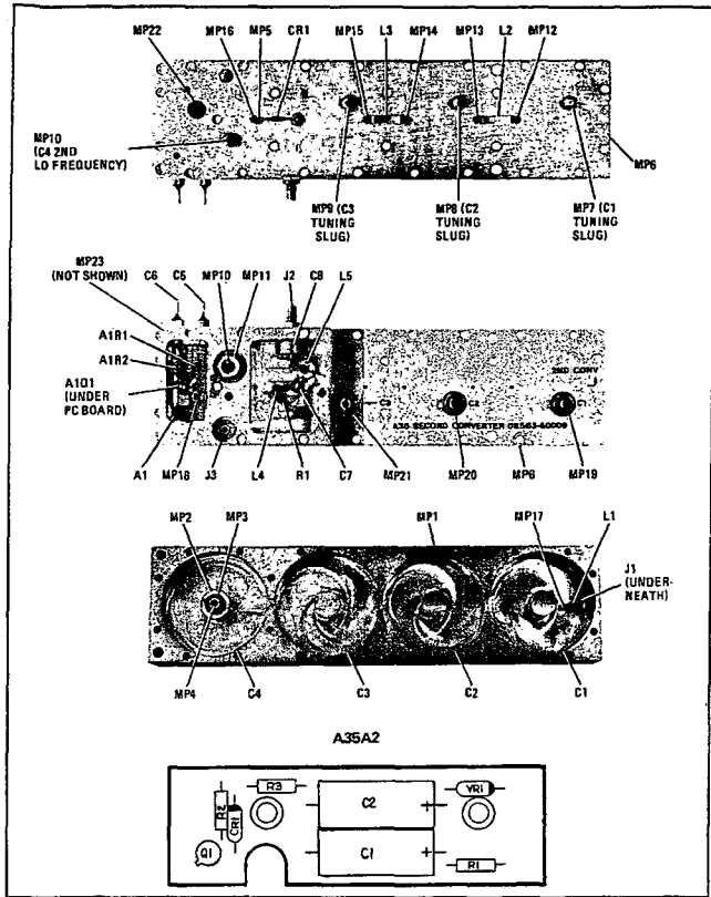
Figure 8-96. A35 Second Converter Assembly, Component Locations
