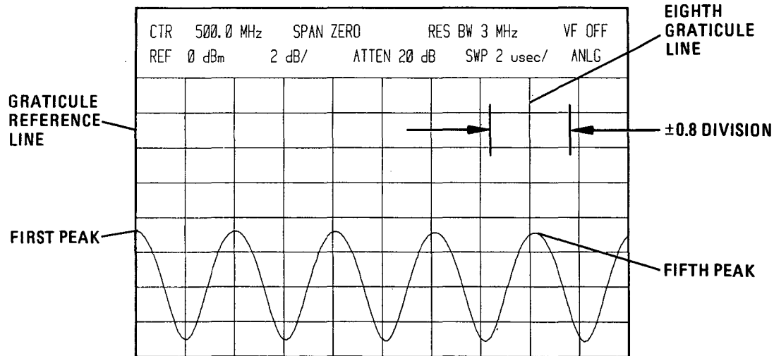
Figure 4-22. Sweep Time Accuracy, 2 \mu SEC/DIV
