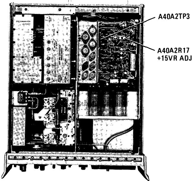
Figure 5-2. A40A2 Adjustment Locations
