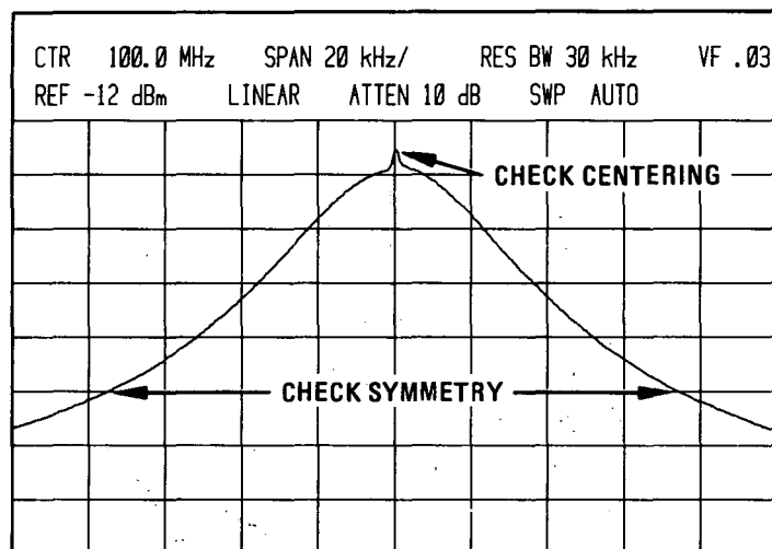
Figure 5-21. Crystal Filter Adjustment
