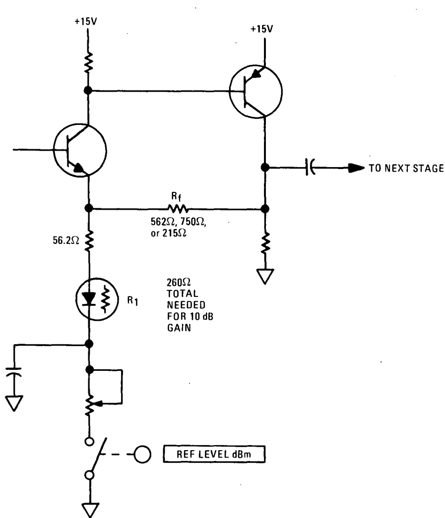
Figure 8-77. Step Gain Amplifiers, Equivalent Circuit
