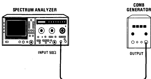
Figure 4-10. Noise Sidebands Test Setup
