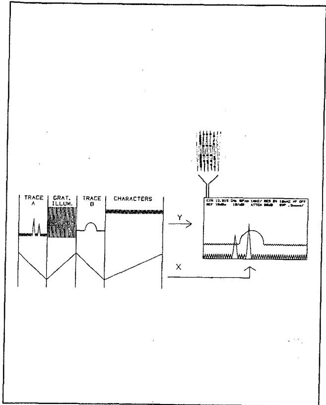
Figure 8-7. Display Refresh Waveforms
