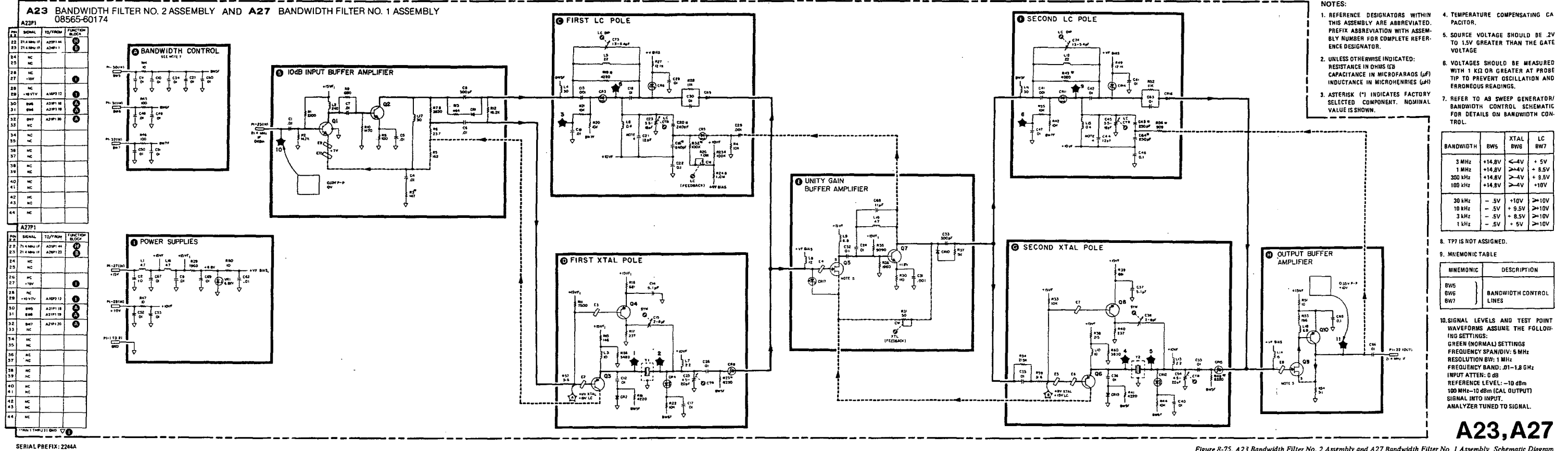
Figure 8-75. A23 Bandwidth Filter No. 2 Assembly and A27 Bandwidth Filter No. 1 Assembly, Schematic Diagram
