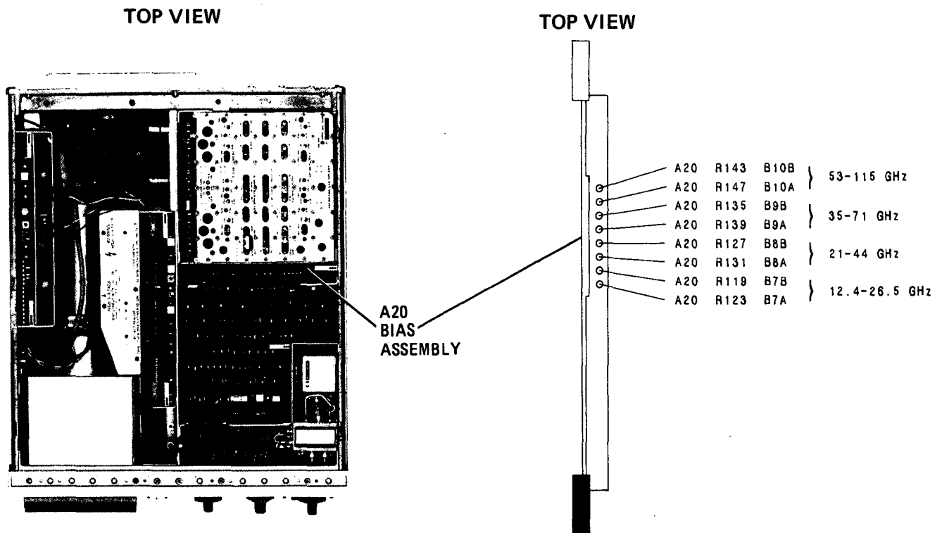
Figure 5-59. Amplitude Calibration of External Mixing Bands Adjustment Locations
