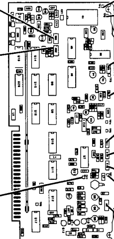
Figure 5-13. Digital Storage Adjustment Locations
