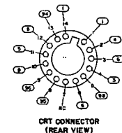
Figure 8-20. A6 High Voltage Power Supply Assembly, Schematic Diagram
