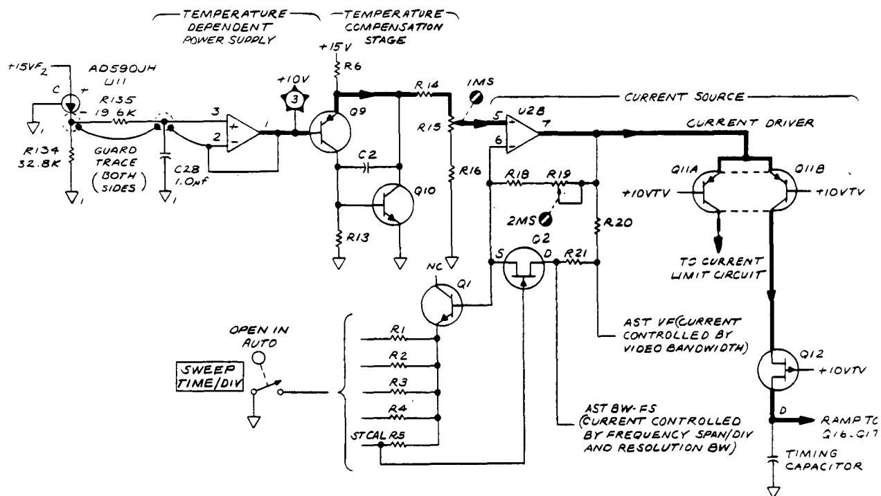
FIGURE 8-50. SIMPLIFIED CIRCUIT FOR SWEEP GENERATOR CURRENT SOURCE (SERIAL PREFIX 2514A)
