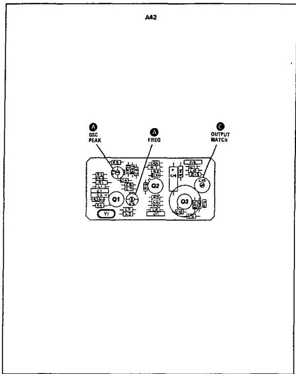
Figure 8-112. Comb Generator Assembly (Option 001), Component Locations
