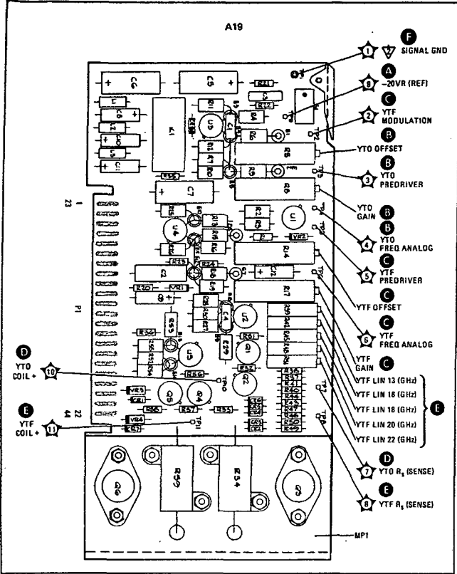
Figure 8-61. A19 YIG Driver Assembly, Component Locations
