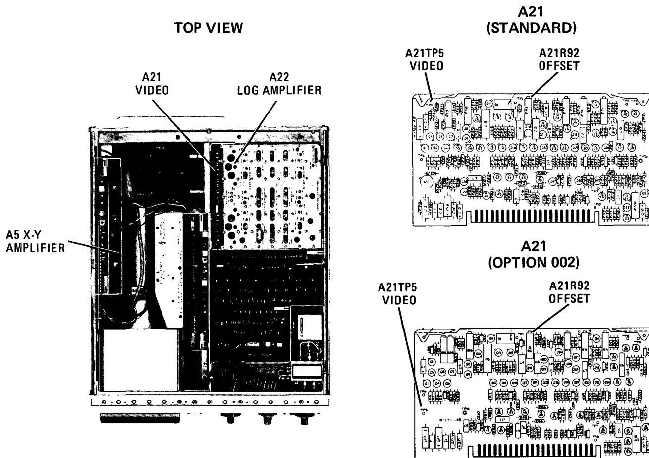
Figure 7-2. Video Offset Adjustment Locations
