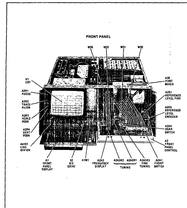
Figure 8-118. HP Model 8569B Major Assembly and Component Locations, Front Panel
