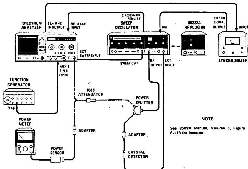
Figure 4-34. Frequency Response Test Setup (internal mixing bands)
