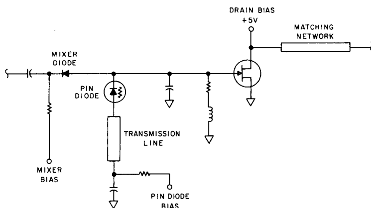
Figure 8-94. A30 First Mixer Assembly, Simplified Schematic
