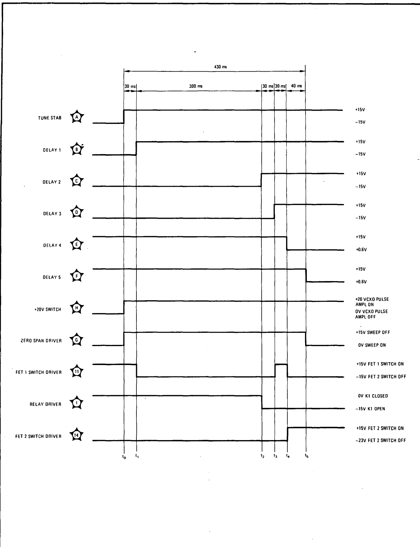
Figure 8-44. Control Generator Timing Diagram (2 of 2)
