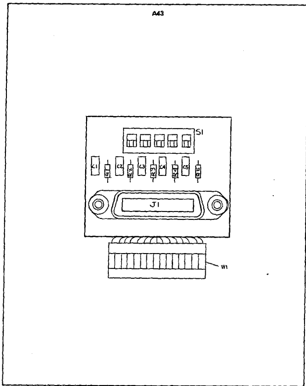
Figure 8-115. A43 HP-IB Connector Assembly, Component Locations
