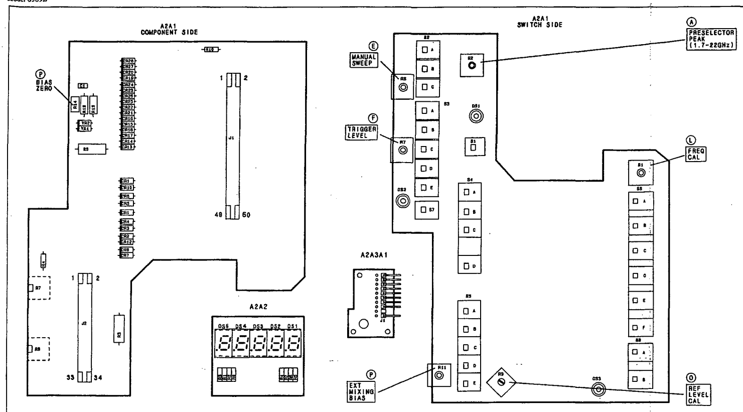
Figure 8-12. A2A1 Front Switch Assembly, A2A2 Frequency Display Assembly, and A2A3A1 Tuning Innerconnect, Component Locations
