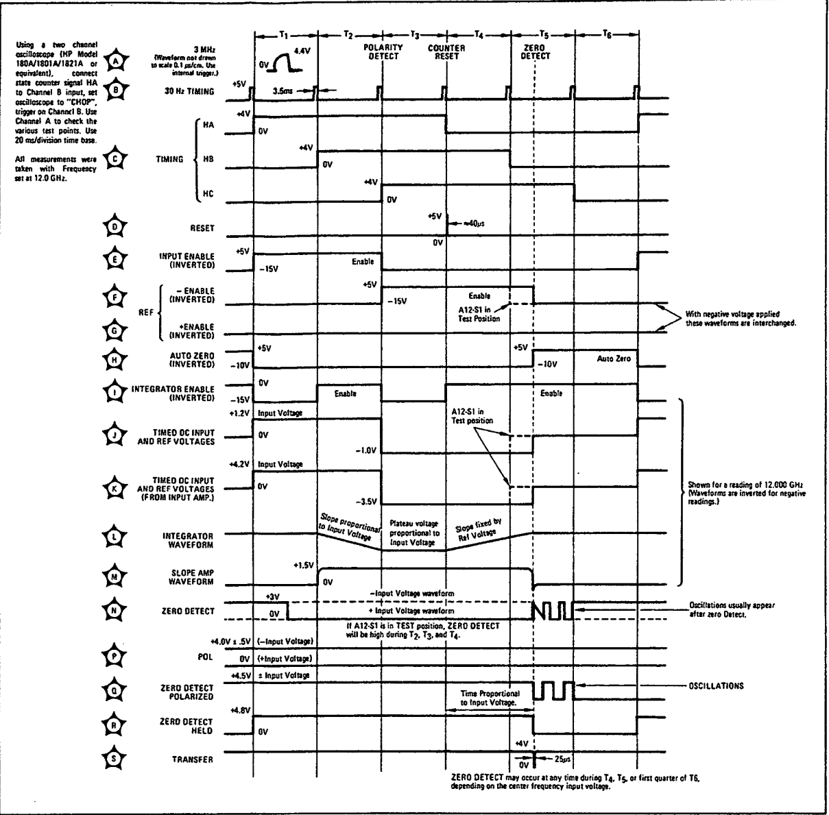
Figure 8-35. Measurement Timing Diagram for A11 DVM Digital Assembly and A12 DVM Analog Assembly
