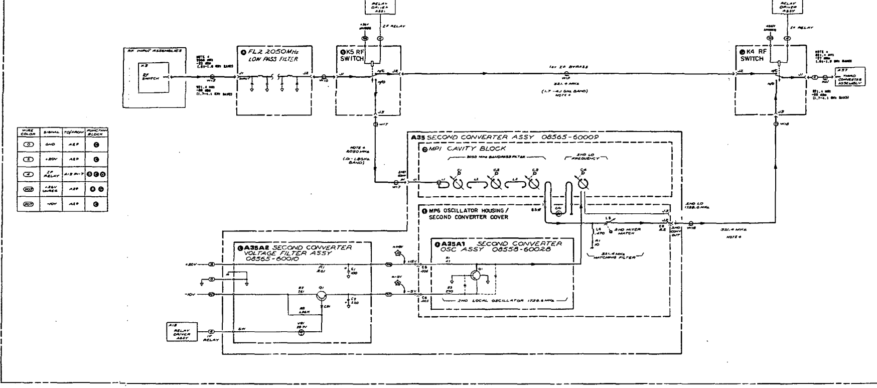
Figure 8-97. A35 Second Converter Assembly, Schematic Diagram
