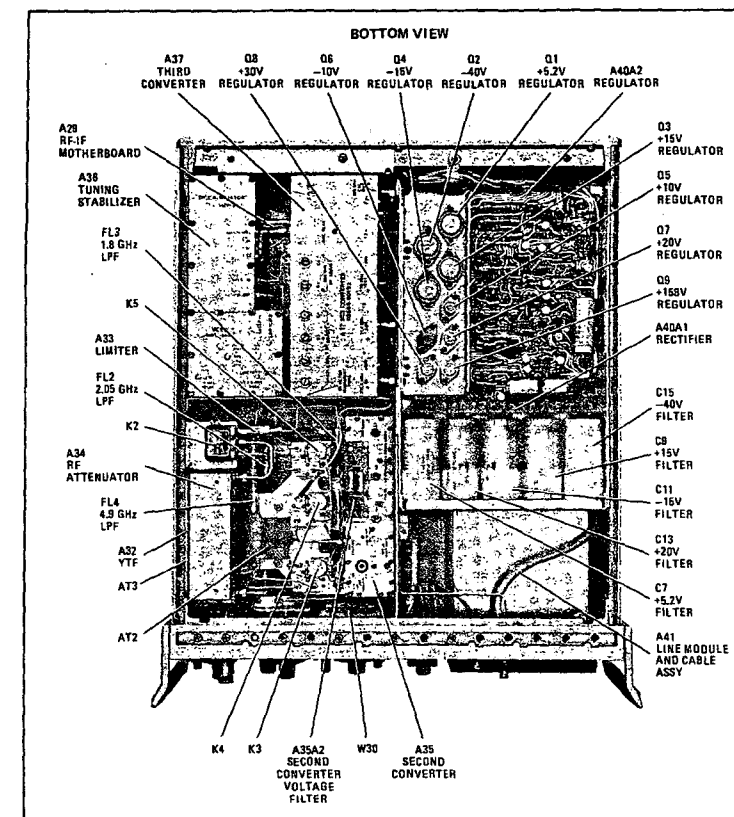
Figure 8-119. HP Model 8569B Major Assembly and Component Locations, Bottom View
