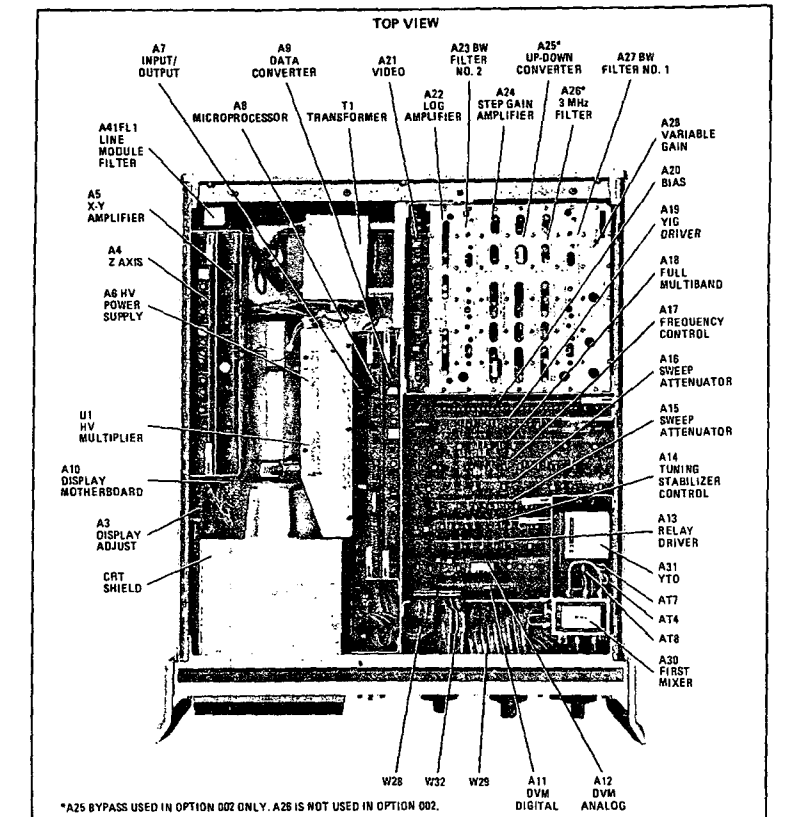
Figure 8-120. HP Model 8569B Major Assembly and Component Locations, Top View
