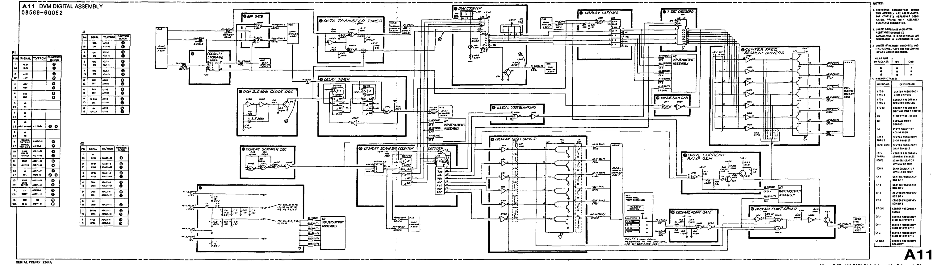
Figure 8-37. A11 DVM Digital Assembly, Schematic Diagram
