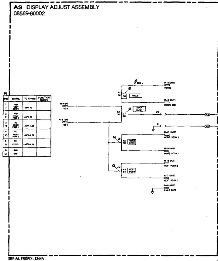
Figure 8-11. A1 Front Panel Display Assembly and A3 Display Adjust Assembly, Schematic Diagram
