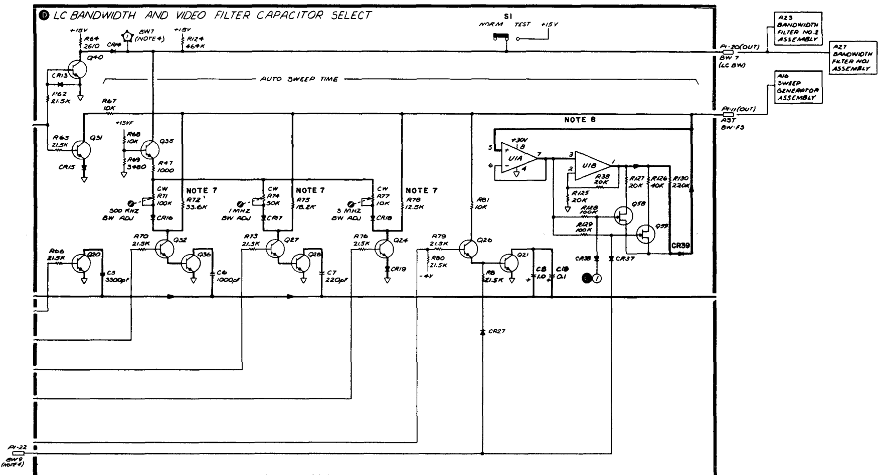
Figure 7-7. P/O A21 Video—100 Hz Assembly, Schematic Diagram (2 of 2)
