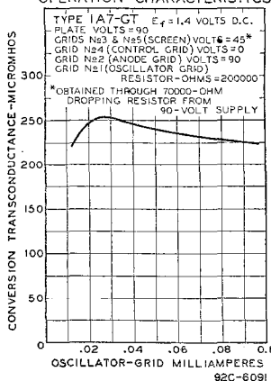
OPERATION CHARACTERISTICS
