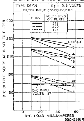
OPERATION CHARACTERISTICS
