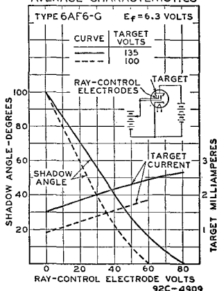
AVERAGE CHARACTERISTICS
