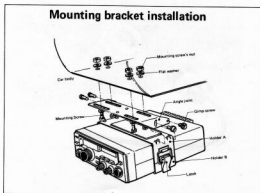
Mounting bracket installation
