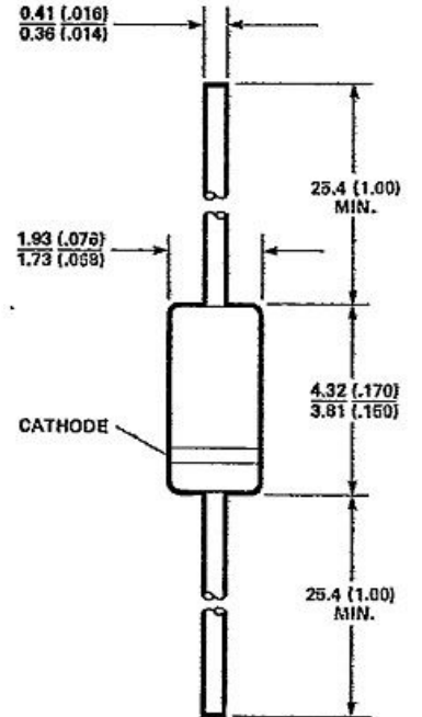
DIMENSIONS IN MILLIMETERS AND (INCHES).
