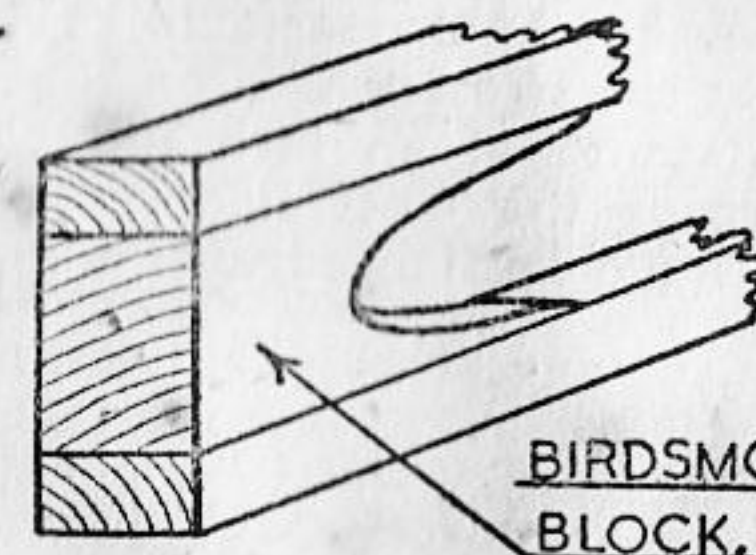
BLOCKED JOINT.
