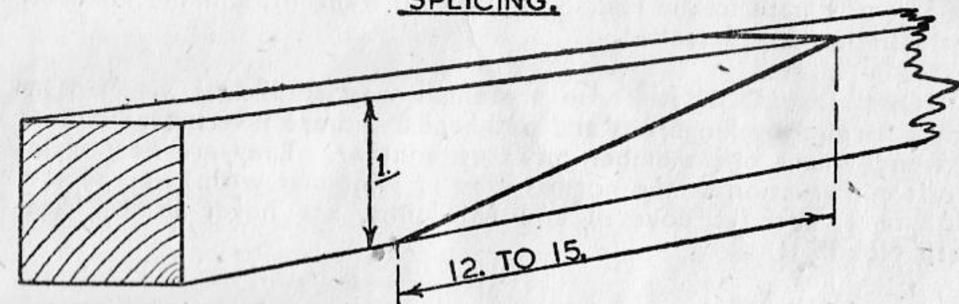
SPLICING.
