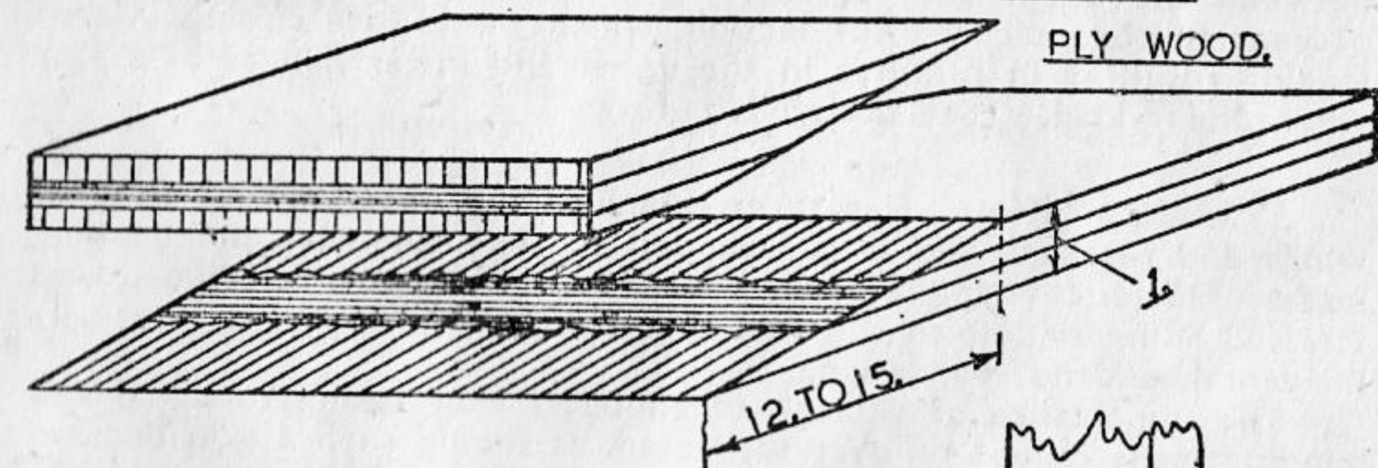
SPLICING.
