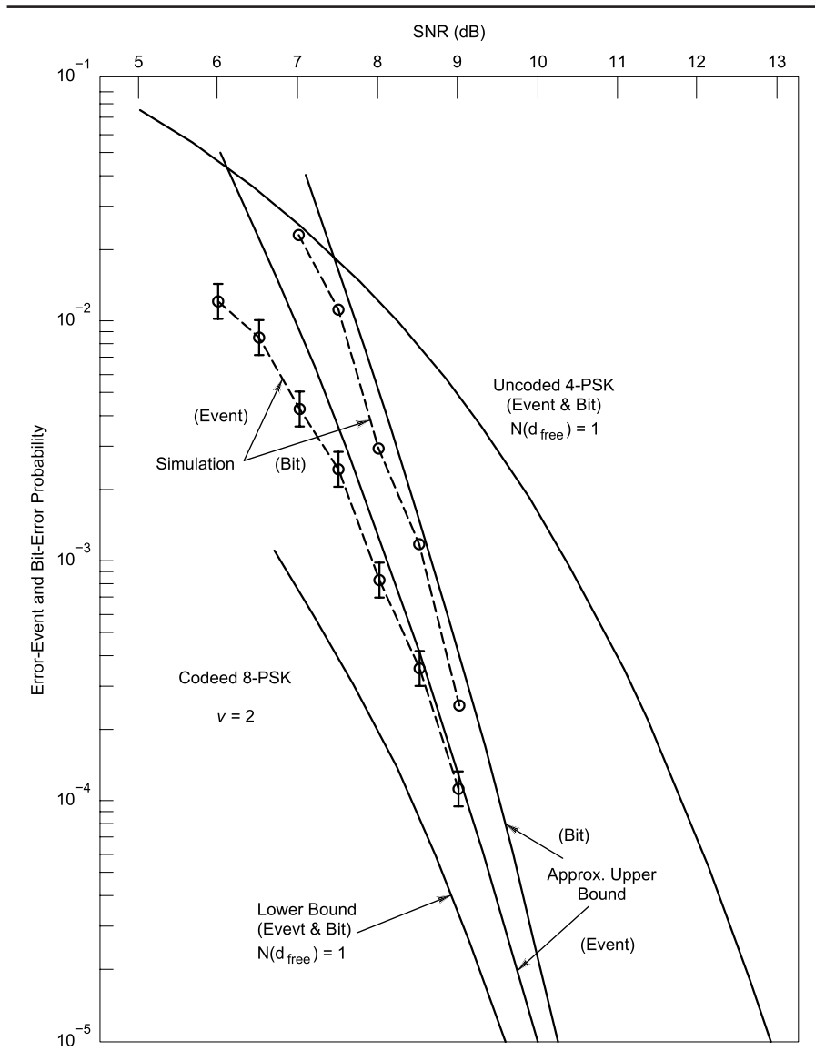
Fig 9—TC8PSK vs. QPSK
