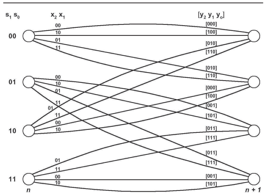
Fig 7—Allowed State Transitions
