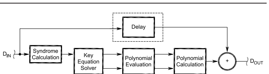
Fig 16—RS Error Correction Process
