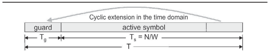
Fig 3—Guard Band
