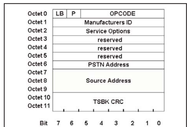
Figure 26: The PSTN Request Message
