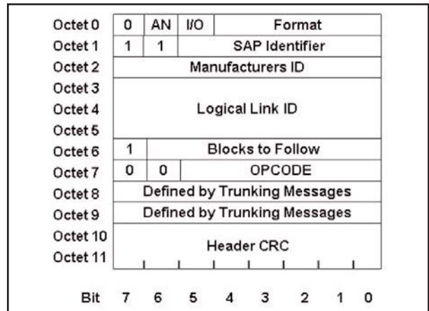
Figure 3: Alternative Trunking Control Packet Header Block
