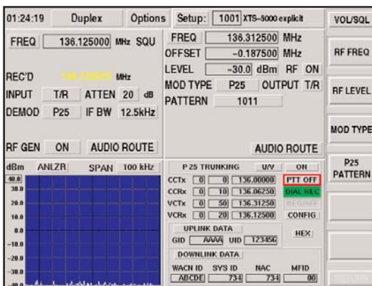
Figure 46: The 2975 Displaying the Dial Request Received from the SU during a PSTN Dial Call
