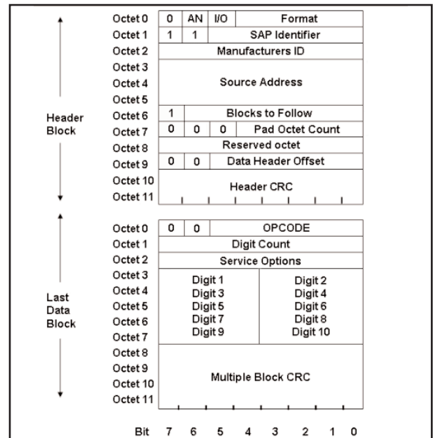
Figure 25: The TELE_INT_DIAL_REQ Message
