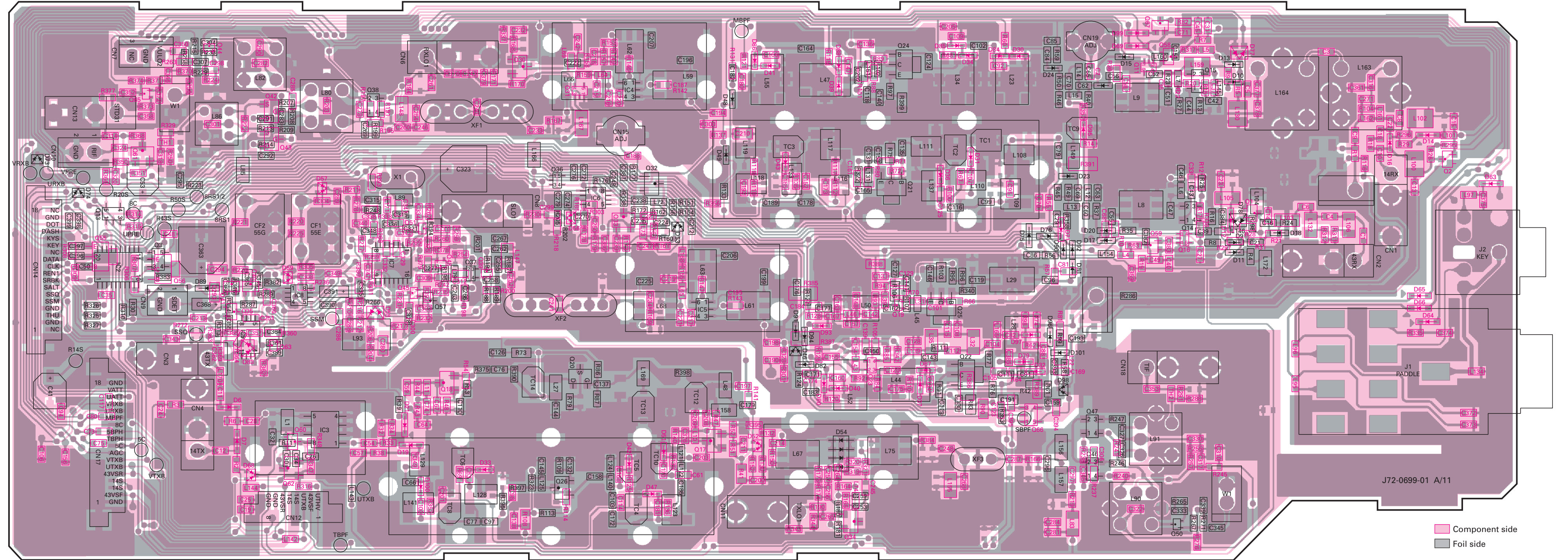
TX-RX 2 UNIT (X57-606X-XX) (A/11) 0-11 : K,KX 2-71 : E,E2 Component side view
