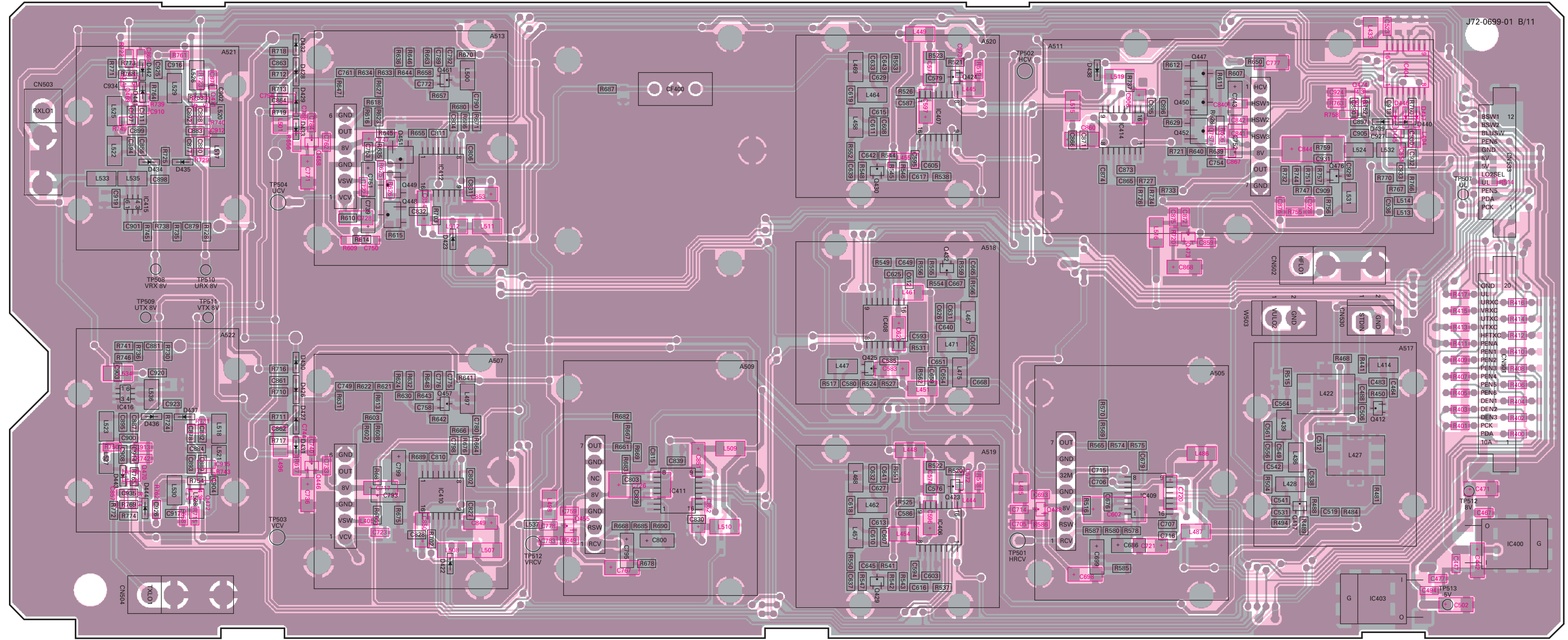
TX-RX 2 UNIT (X57-606X-XX) (B/11) 0-11 : K,KX 2-71 : E,E2 Foil side view
