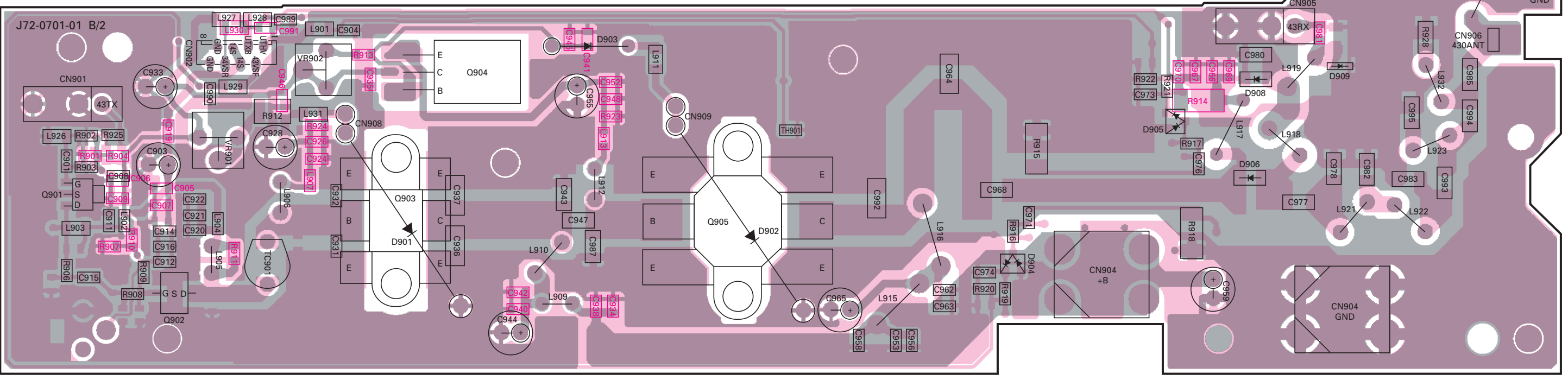
FIANL UNIT (X45-360X-XX) (B/2) 0-11 : K,KX 2-71 : E,E2 Component side view
